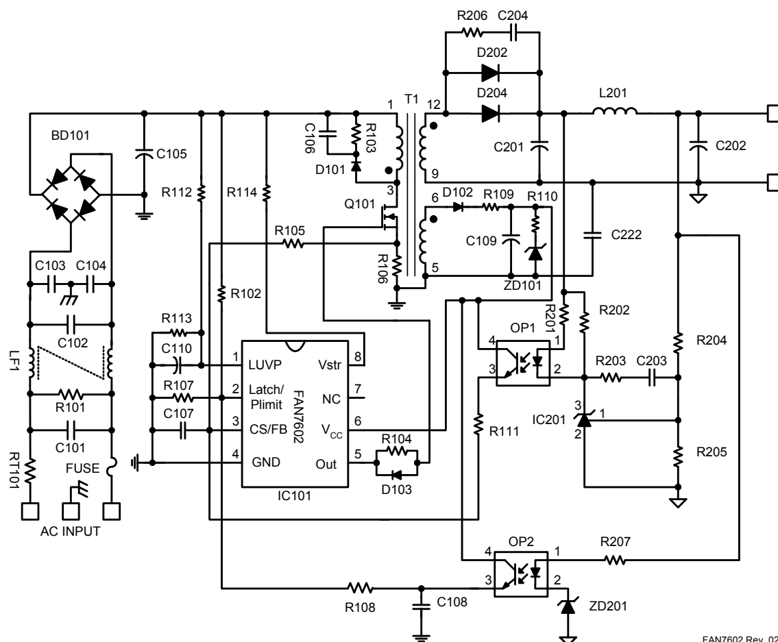
Figure 26. Schematic
