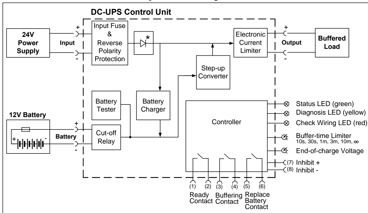
Fig. 11-1 Functional diagram
