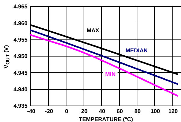
FIGURE 31. V_{OUT} HIGH vs TEMPERATURE, V_+ = 5V , V_- = 0V , V_{CM} = 2.5V , R_L = 1k
