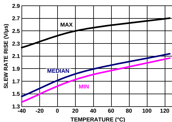
FIGURE 35. SLEW RATE RISE vs TEMPERATURE, V_{OUT} = \pm 1.5V , V_{P-P} V_+ , V_- = 0V , V_{CM} = 2.5V , R_L = 100k
