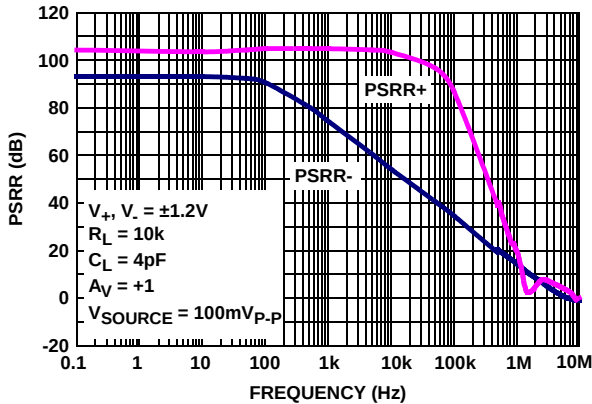
FIGURE 9. PSRR vs FREQUENCY, V_+, V_- = \pm 1.2V
