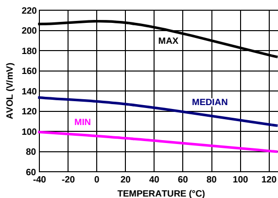
FIGURE 30. AVOL vs TEMPERATURE, V_+ , V_- = \pm 2.5V , V_O = -2V \text{ TO } +2V , R_L = 1k
