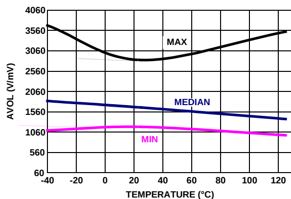
FIGURE 29. AVOL vs TEMPERATURE, V_+ , V_- = \pm 2.5V , V_O = -2V \text{ TO } +2V , R_L = 100k
