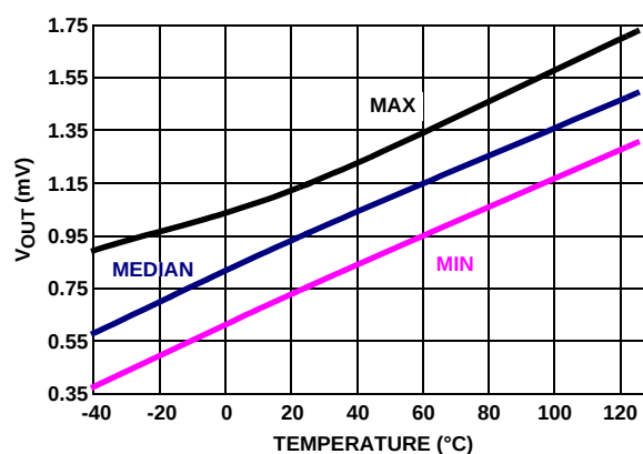
FIGURE 34. V_{OUT} LOW vs TEMPERATURE, V_+ = 5V , V_- = 0V , V_{CM} = 2.5V , R_L = 100k
