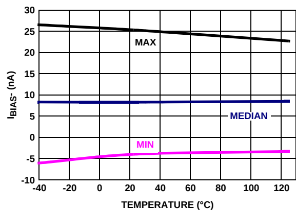
FIGURE 23. I_{BIAS+} vs TEMPERATURE, V_+ , V_- = \pm 1.2V
