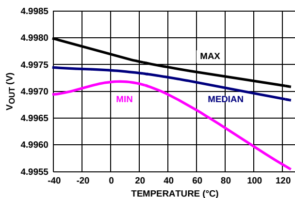
FIGURE 33. V_{OUT} HIGH vs TEMPERATURE, V_+ = 5V , V_- = 0V , V_{CM} = 2.5V , R_L = 100k
