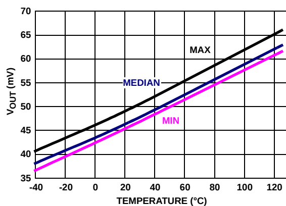
FIGURE 32. V_{OUT} LOW vs TEMPERATURE, V_+ = 5V , V_- = 0V , V_{CM} = 2.5V , R_L = 1k
