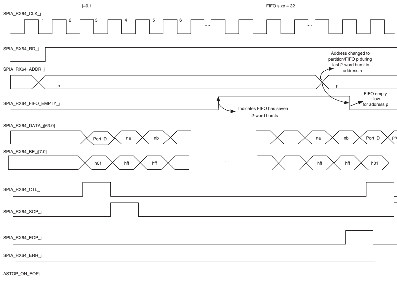
Figure 36. Read Timing with ASTOP_ON_EOP Deasserted - 64-Bit Mode
