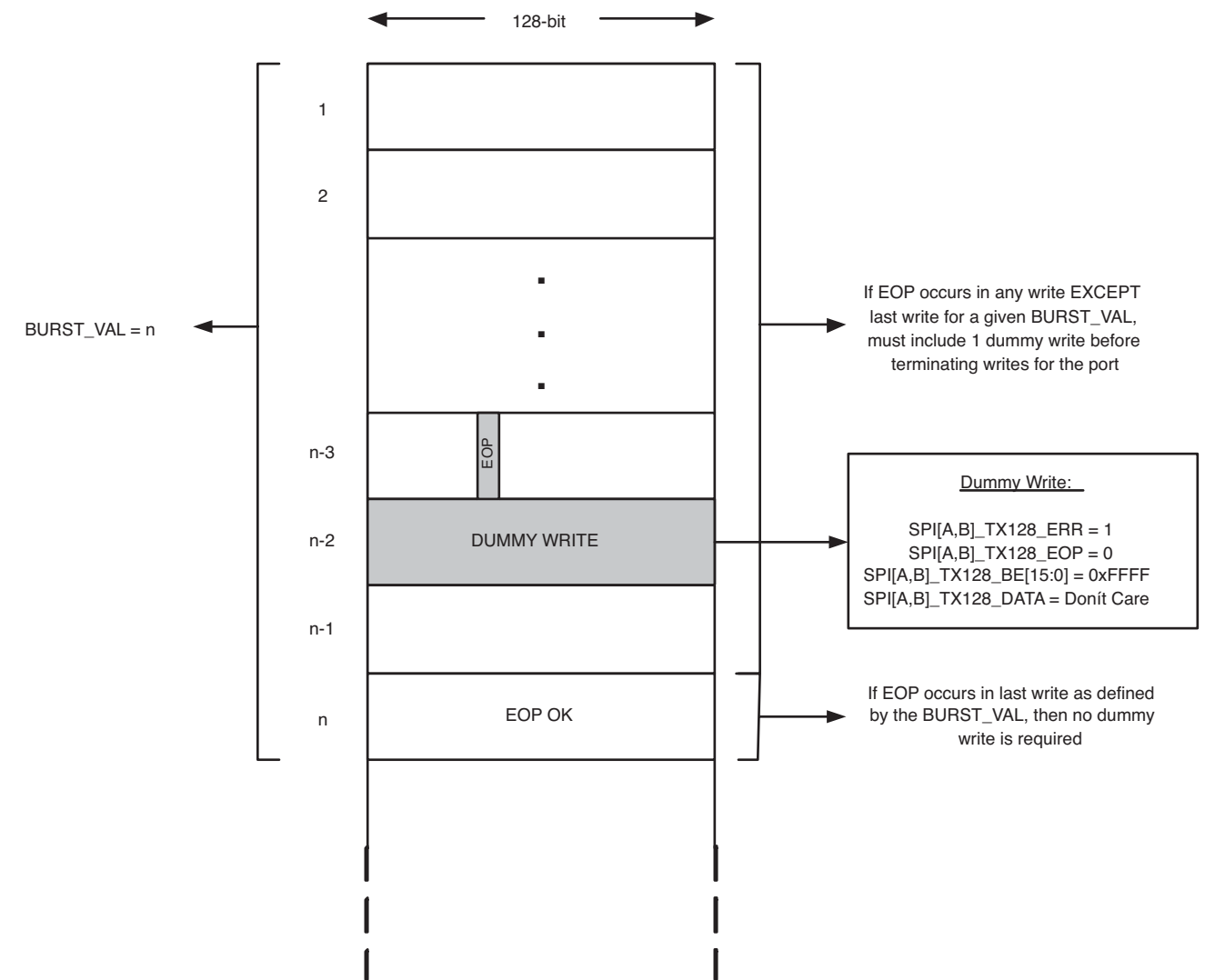
Figure 24. Dummy Write Requirement for MIN_BURST_MODE (128-Bit Mode)
