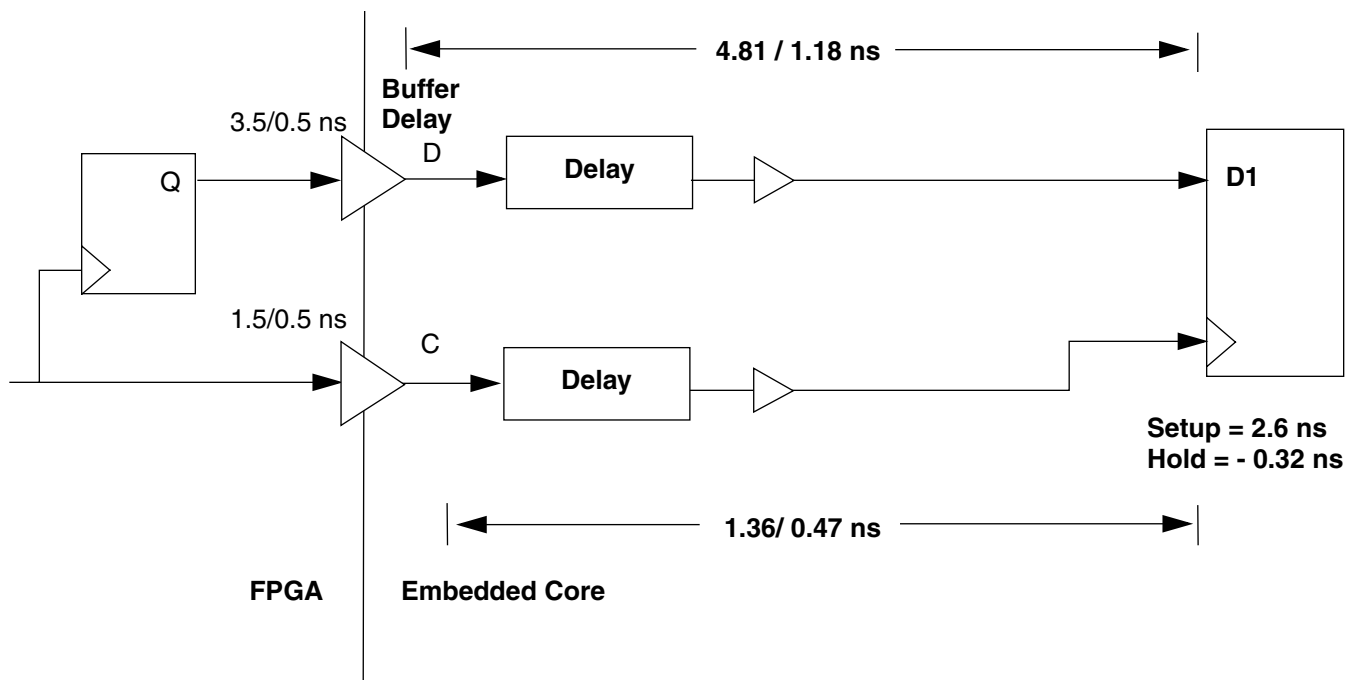
Figure 27. Data: SPI[A,B]_{DATA/SOP/EOP/BE/ERR/PORT/WE/ADDR/SPI[A,B]_{TXk\_WD\_CNT\_RST}/LINK\_DIS
