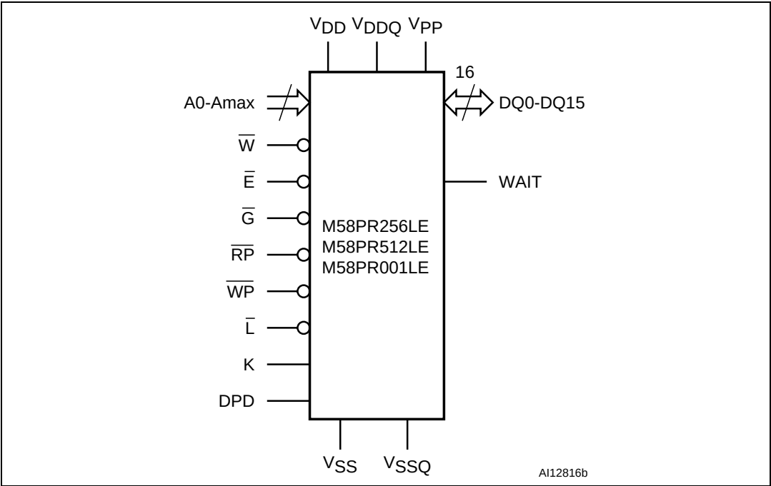
Figure 1. Logic diagram
