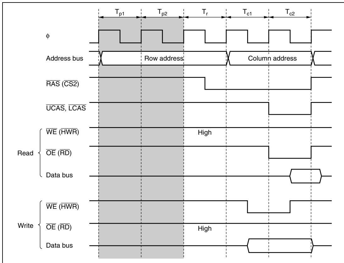
Figure 6.26 Example of Timing with Two-State Precharge Cycle ( \text{RAST} = 0 , \text{CAST} = 0 )
