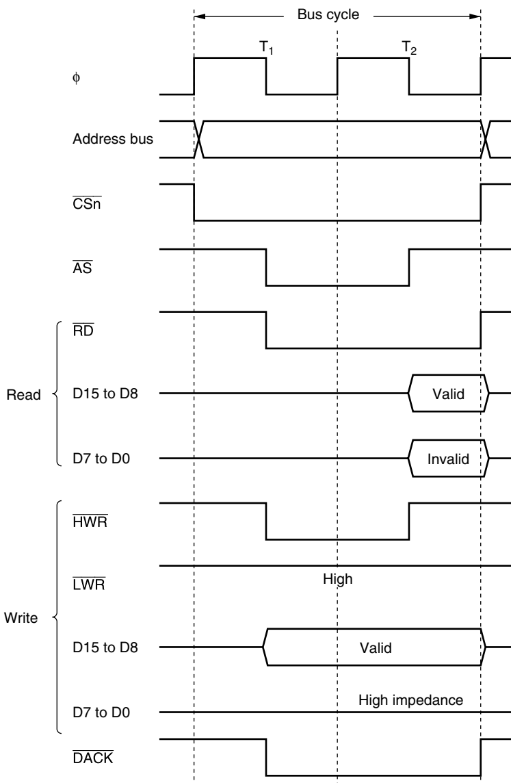
Figure 6.13 Bus Timing for 16-Bit, 2-State Access Space (Even Address Byte Access)
