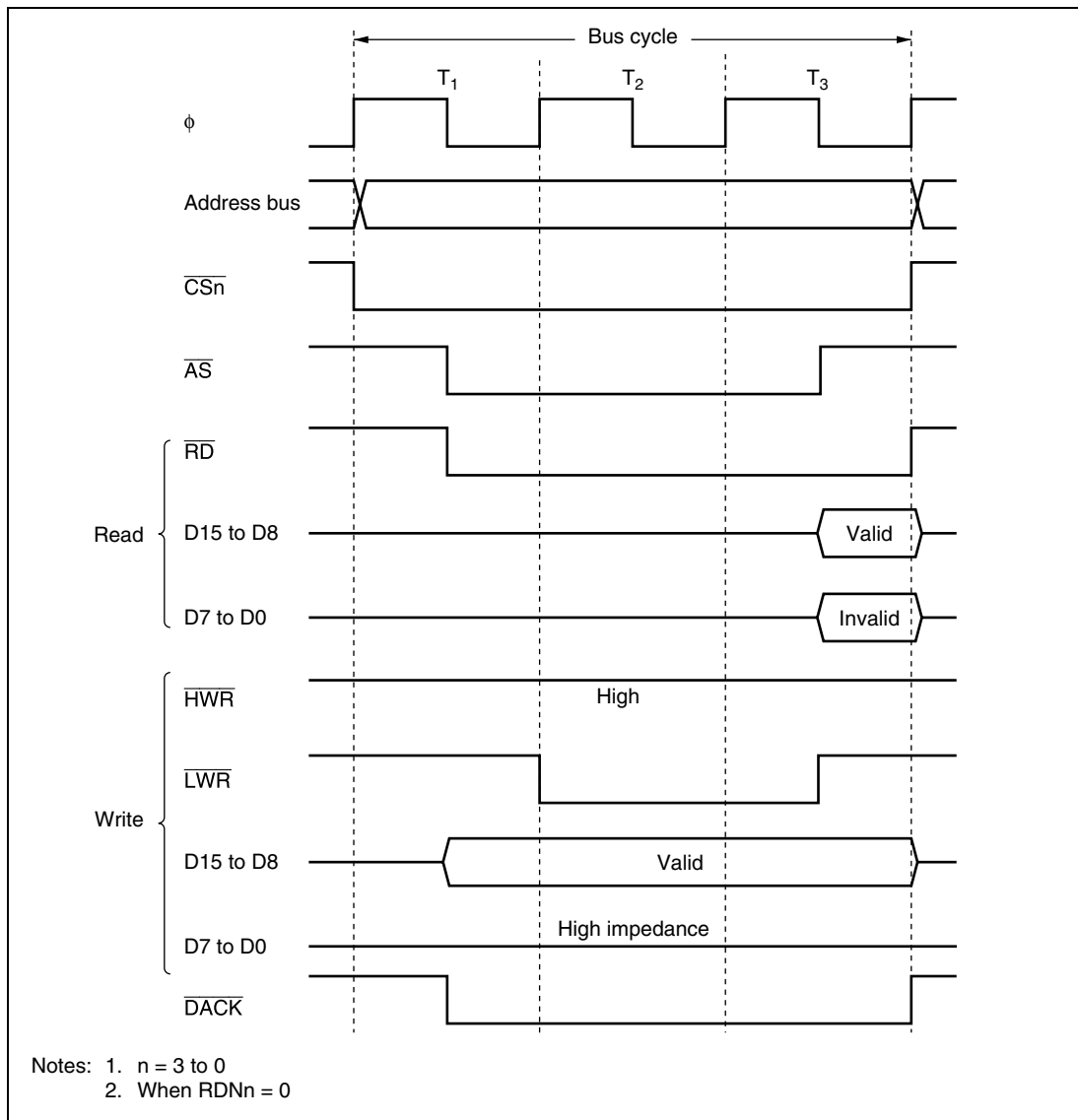
Figure 6.12 Bus Timing for 8-Bit, 3-State Access Space
