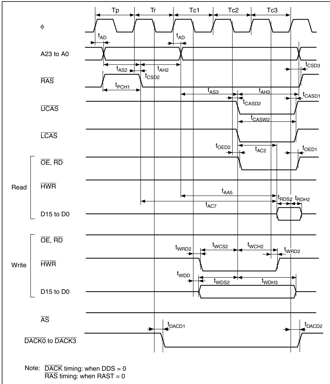
Figure 18.14 DRAM Access Timing: Three-State Access (RAST = 1)
