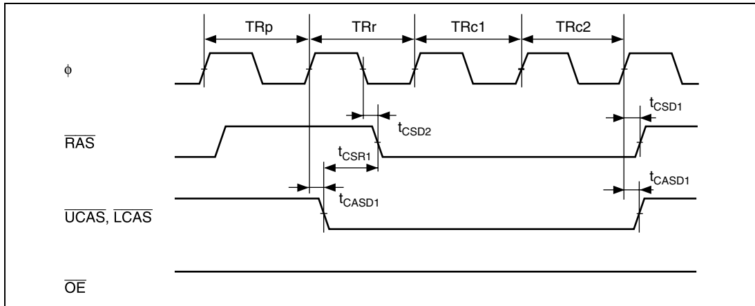
Figure 18.16 CAS-Before-RAS Refresh Timing
