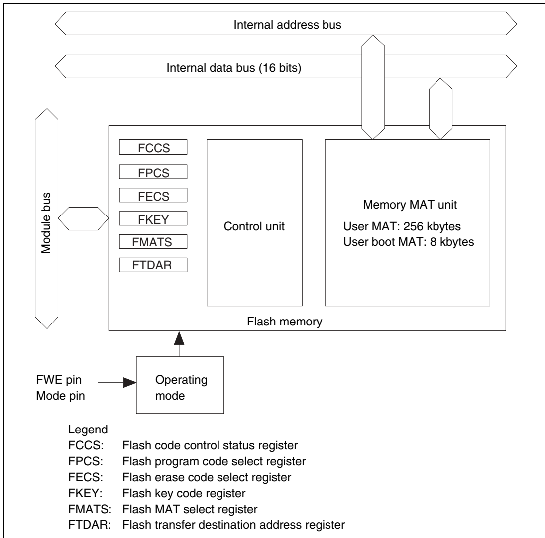
Figure 14.1 Block Diagram of Flash Memory
