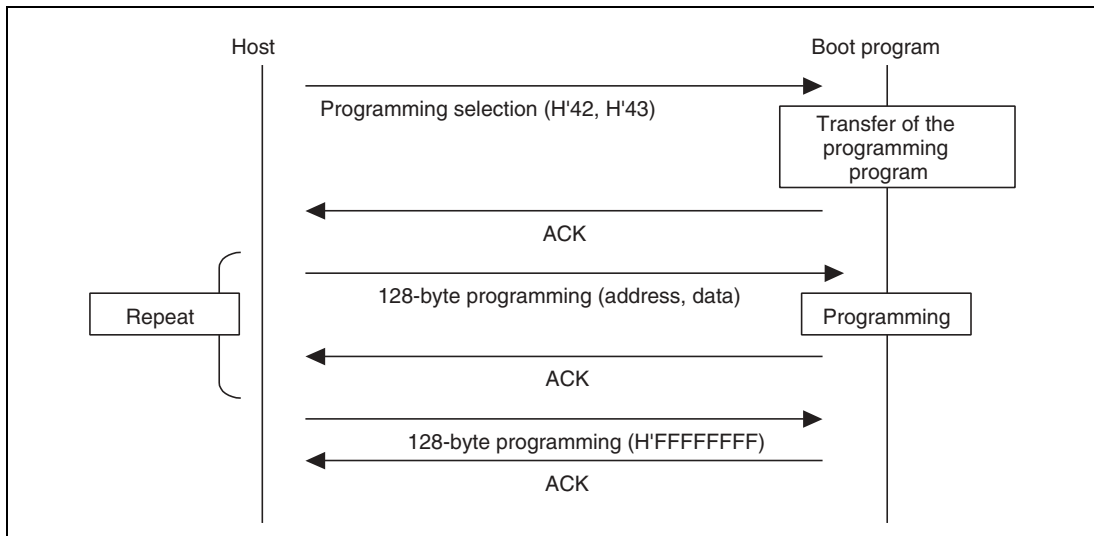
Figure 14.25 Programming Sequence
