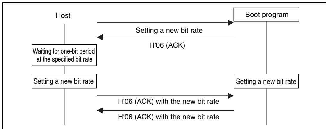
Figure 14.24 New Bit-Rate Selection Sequence
