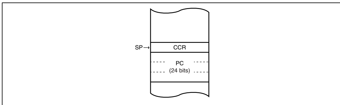
Figure 4.2 Stack Status after Exception Handling
