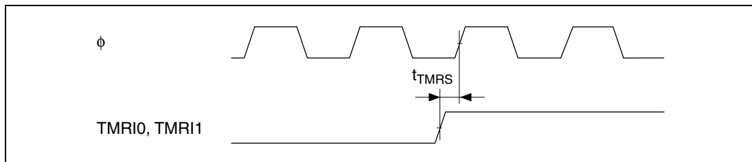
Figure 18.27 8-Bit Timer Reset Input Timing
