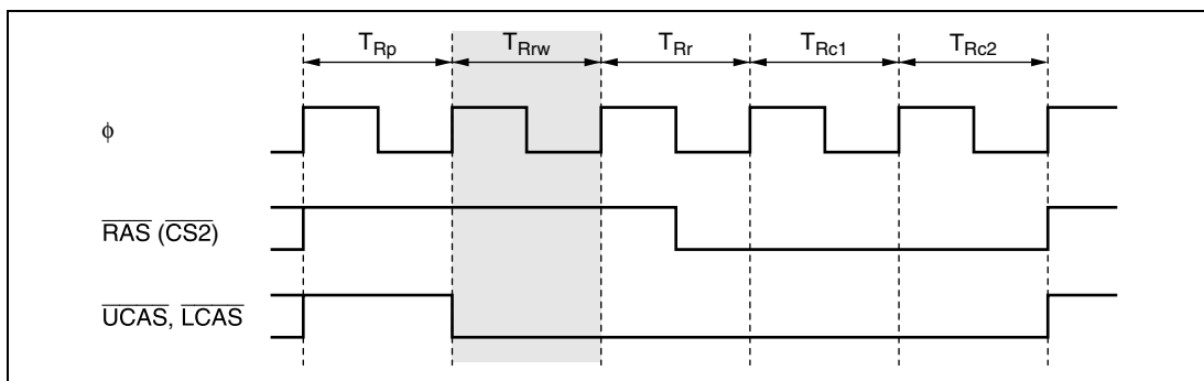
Figure 6.39 CBR Refresh Timing (RCW1 = 0, RCW0 = 1, RLW1 = 0, RLW0 = 0)
