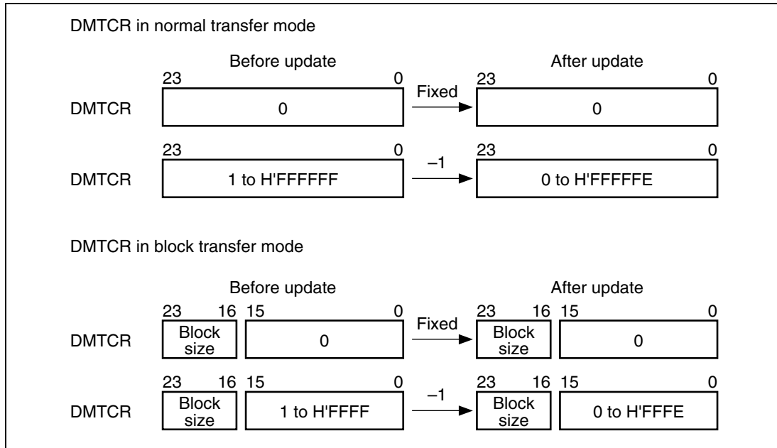
Figure 7.11 DMTCCR Update Operations in Normal Transfer Mode and Block Transfer Mode
