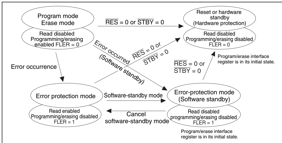
Figure 14.16 Transitions to Error-Protection State
