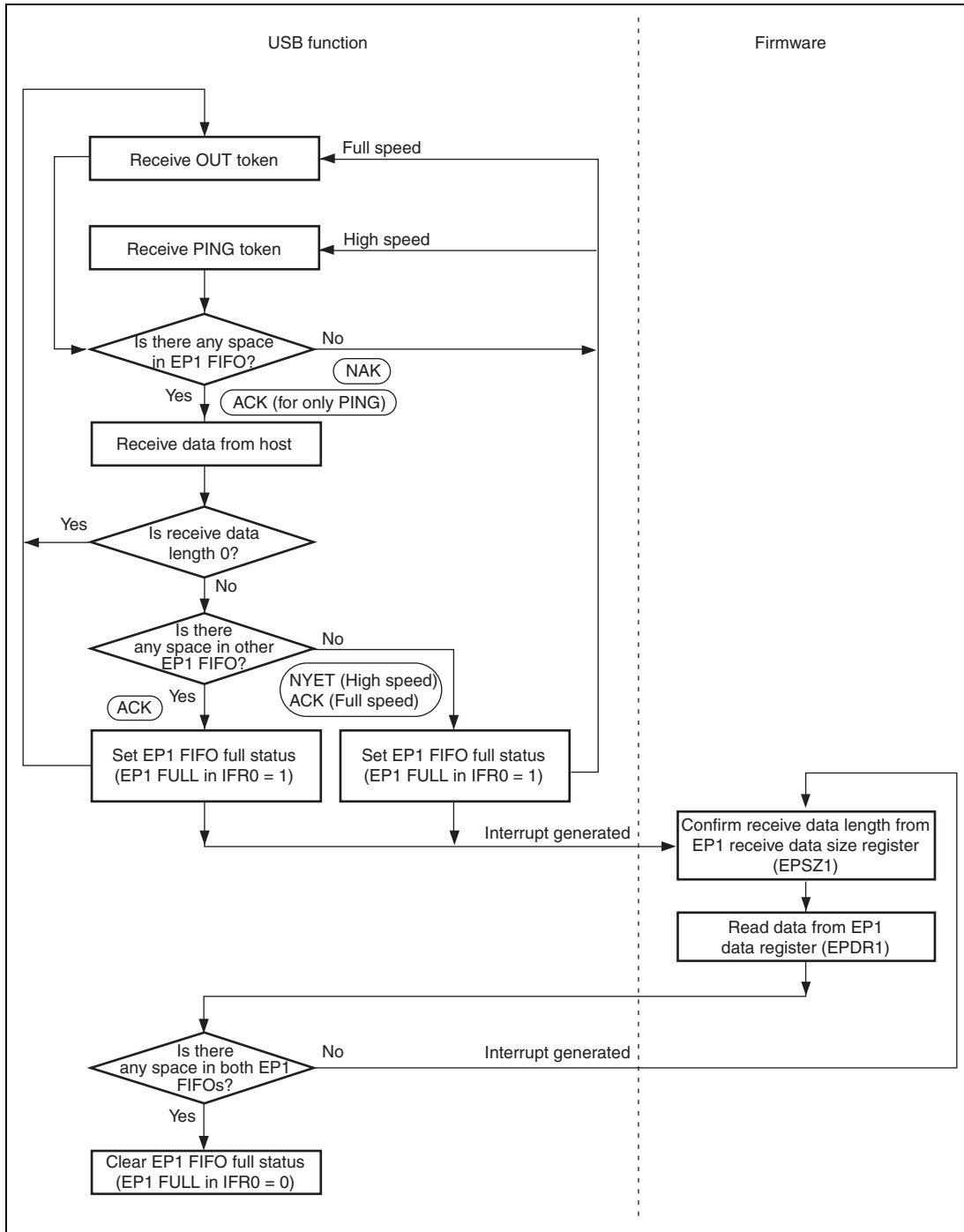
Figure 12.10 EP1 Bulk-Out Transfer Operation
