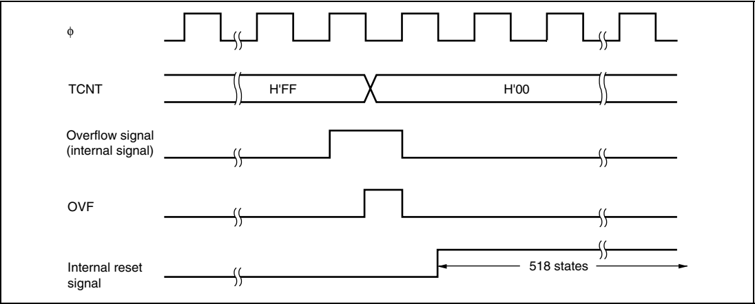
Figure 10.5 Output Timing of OVF
