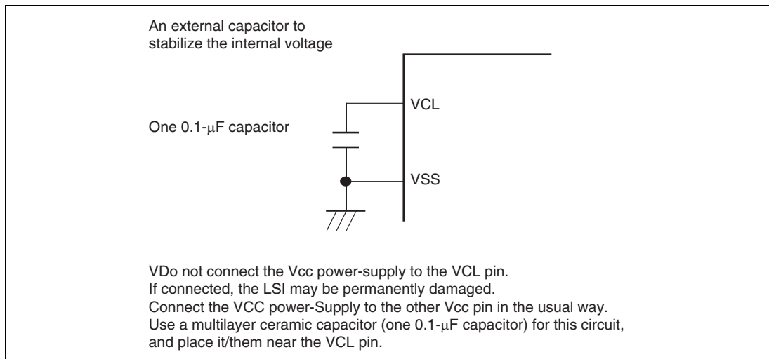
Figure 18.29 VCL Capacitor Connection Method
