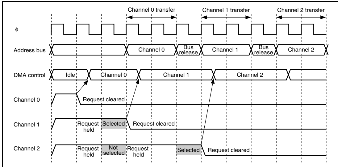
Figure 7.13 Example of Channel Priority Timing
