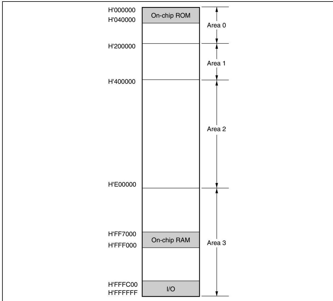
Figure 6.7 Address Map
