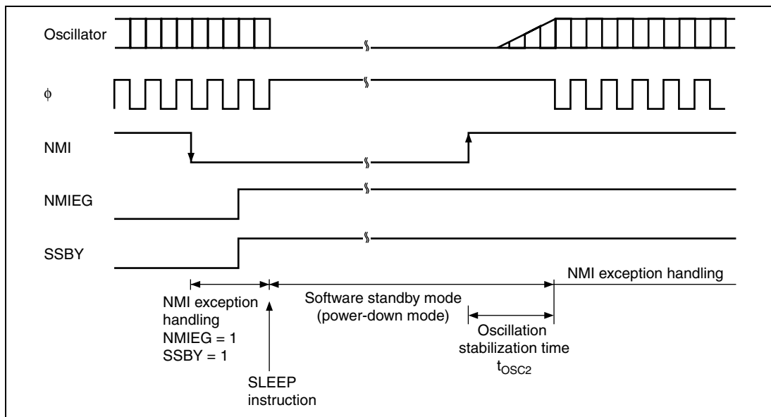
Figure 18.5 Oscillation Stabilization Timing (2)
