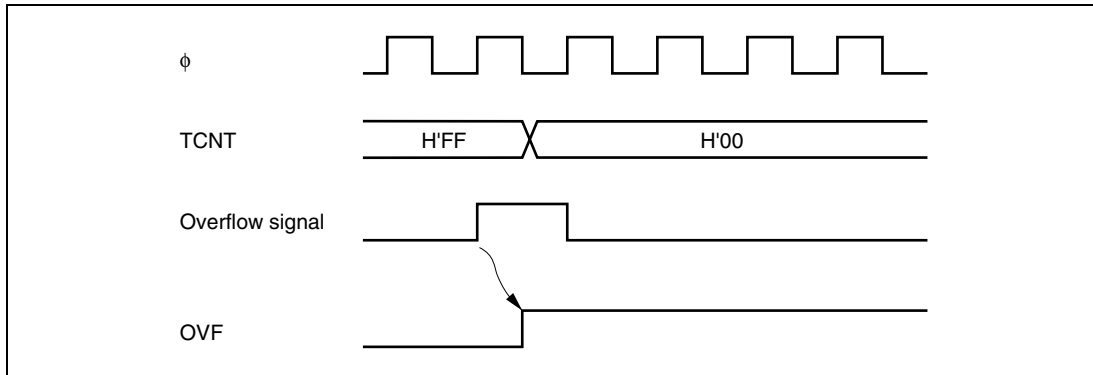
Figure 9.9 Timing of OVF Setting
