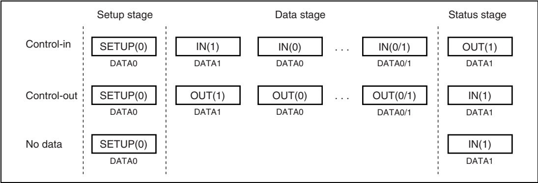
Figure 12.4 Control Transfer Stage Configuration
