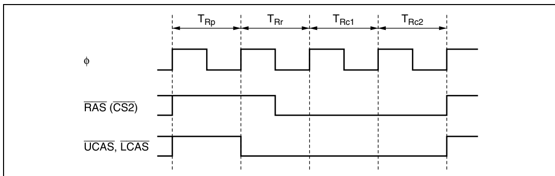
Figure 6.38 CBR Refresh Timing
