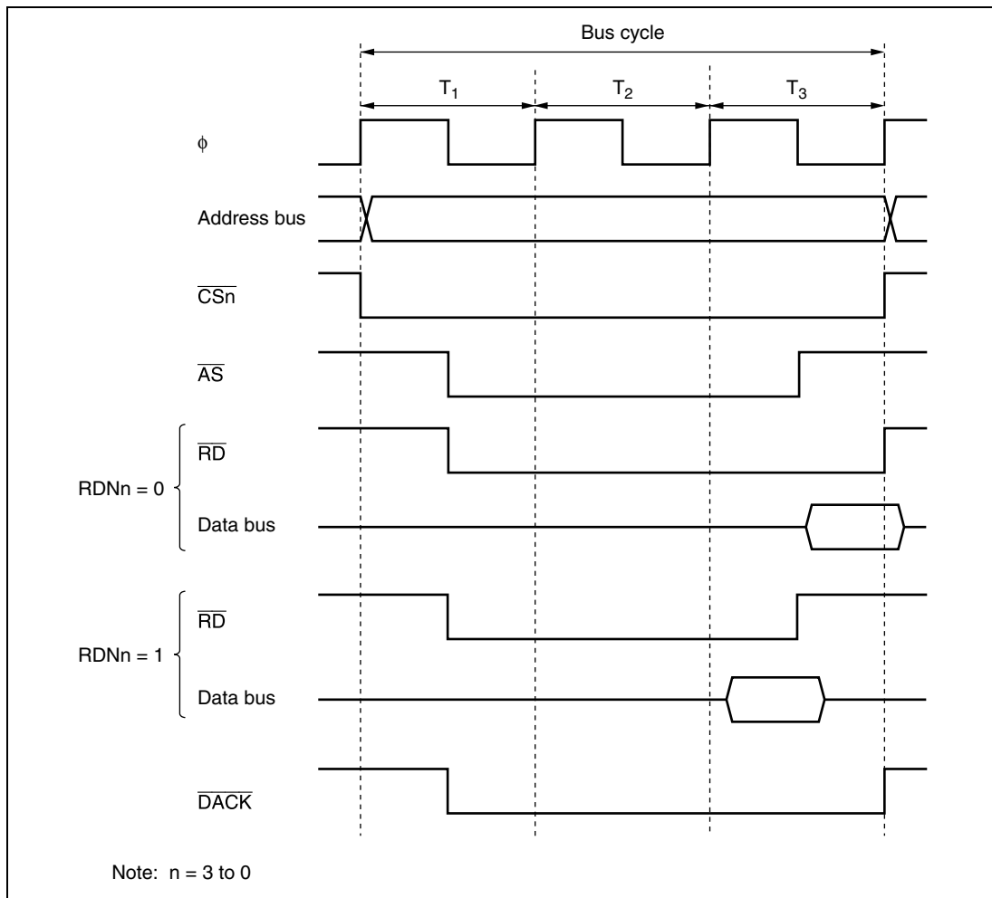
Figure 6.20 Example of Read Strobe Timing
