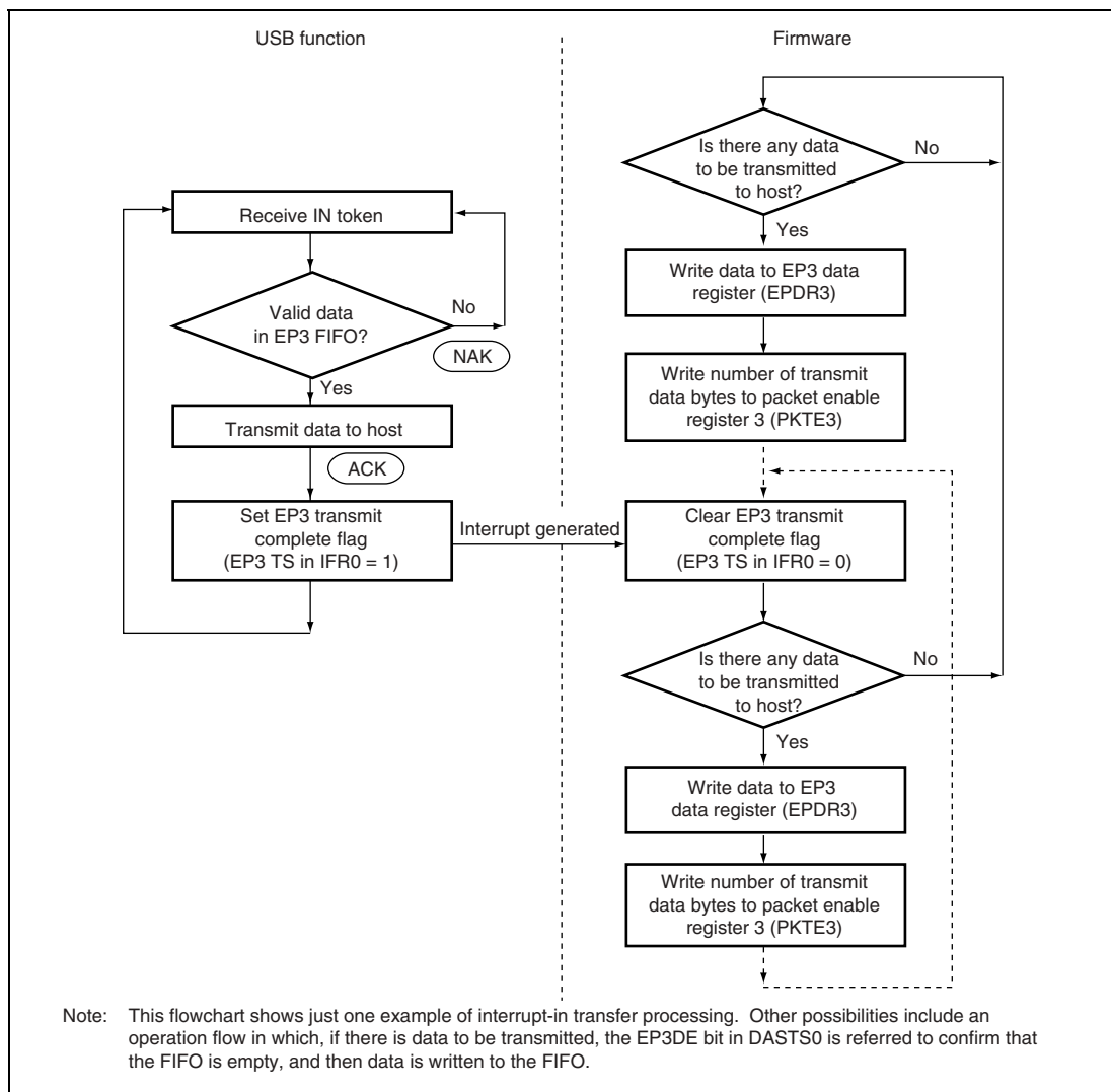
Figure 12.12 EP3 Interrupt-In Transfer Operation
