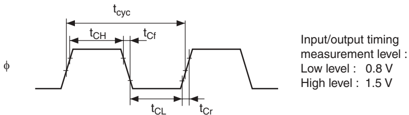
Figure 18.3 System Clock Timing
