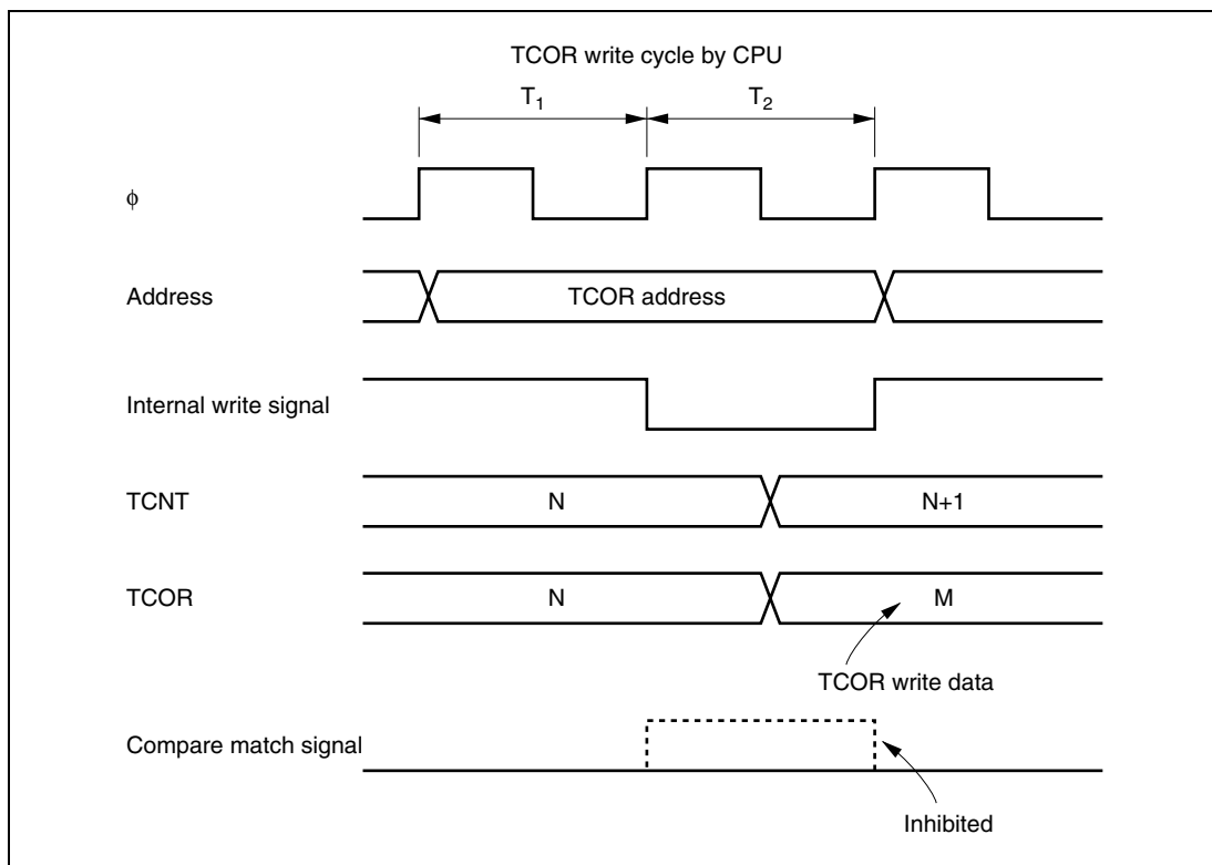
Figure 9.12 Contention between TCOR Write and Compare Match
