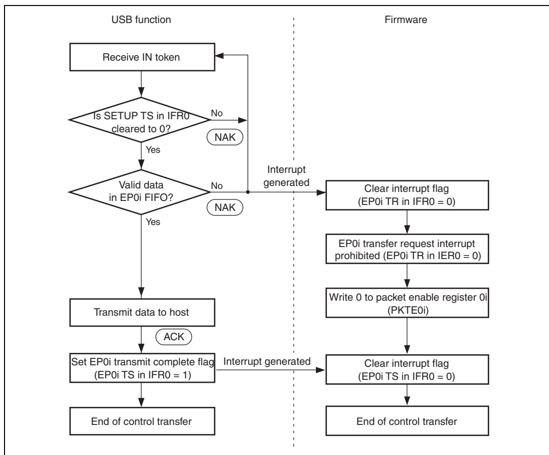
Figure 12.9 Status Stage Operation (Control-Out)
