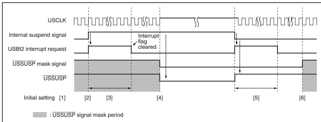
Figure 12.16 Enter/Recover Sequence of USB Suspend State
