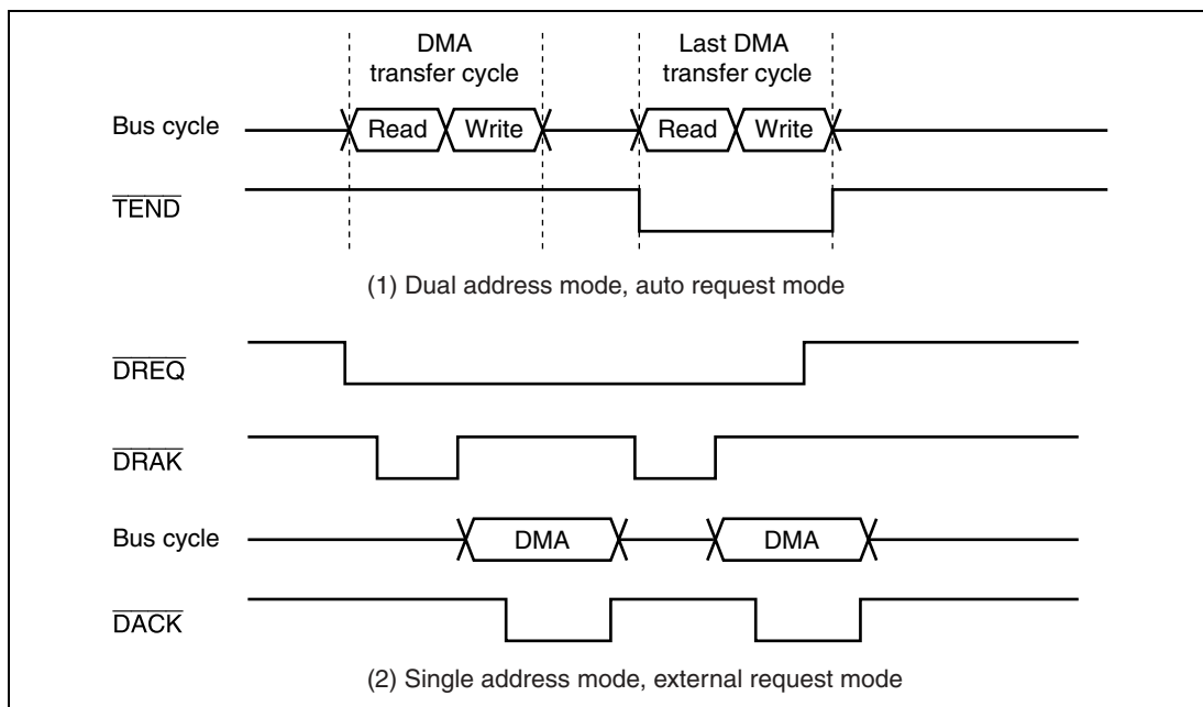
Figure 7.7 Examples of Timing in Normal Transfer Mode
