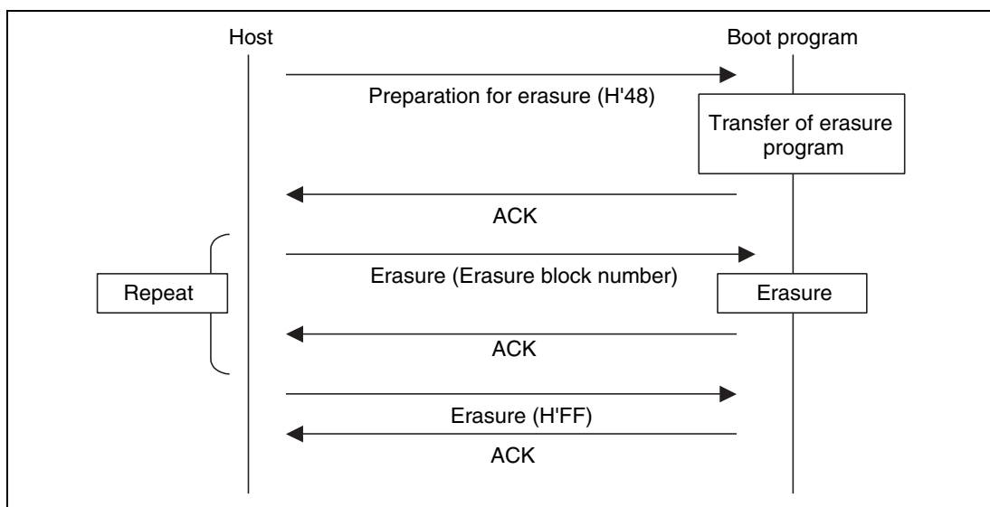
Figure 14.26 Erasure Sequence
