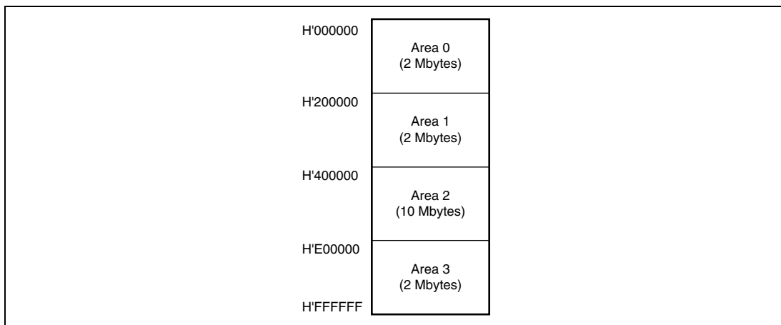
Figure 6.5 Area Divisions
