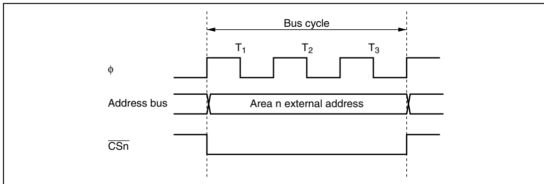
Figure 6.8 \overline{\text{CSn}} Signal Output Timing (n = 3 to 0)
