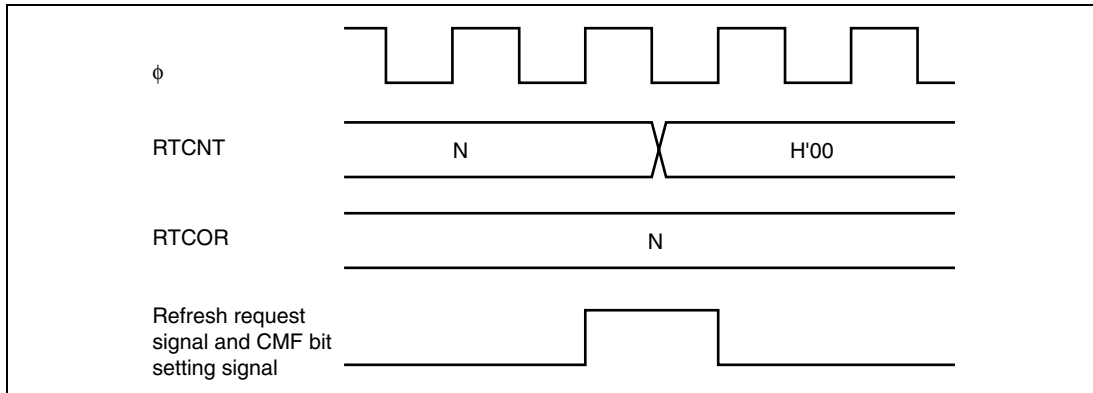
Figure 6.37 Compare Match Timing
