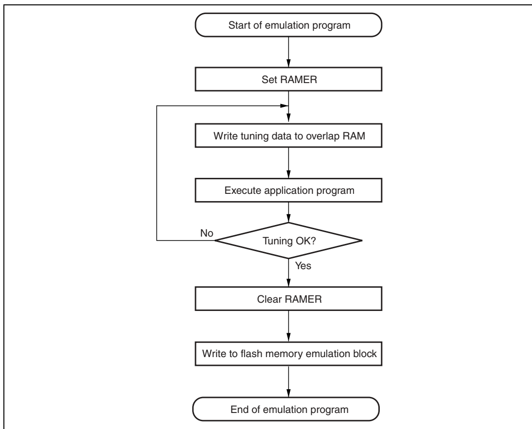
Figure 14.18 Flowchart for Flash Memory Emulation in RAM
