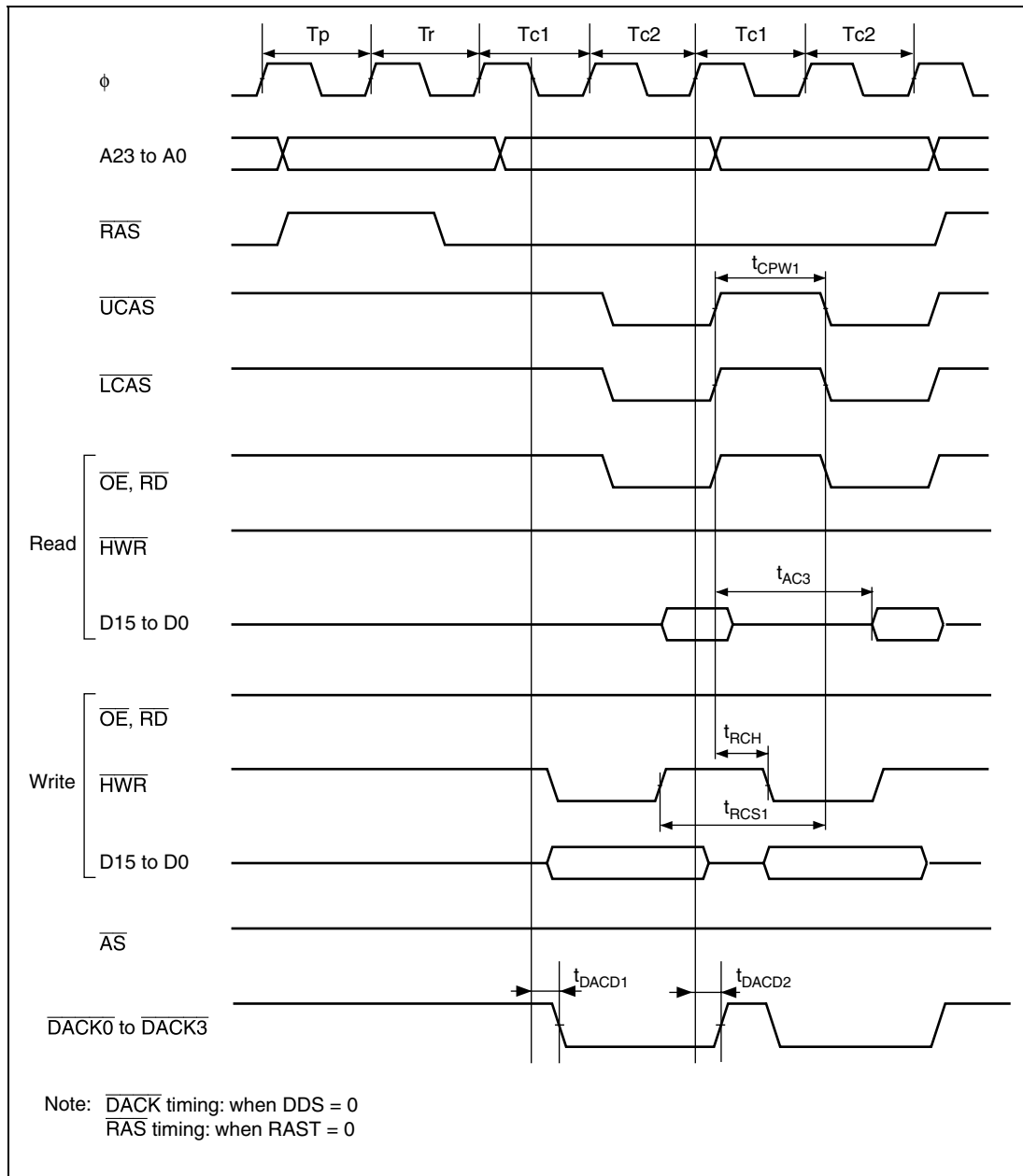
Figure 18.13 DRAM Access Timing: Two-State Burst Access
