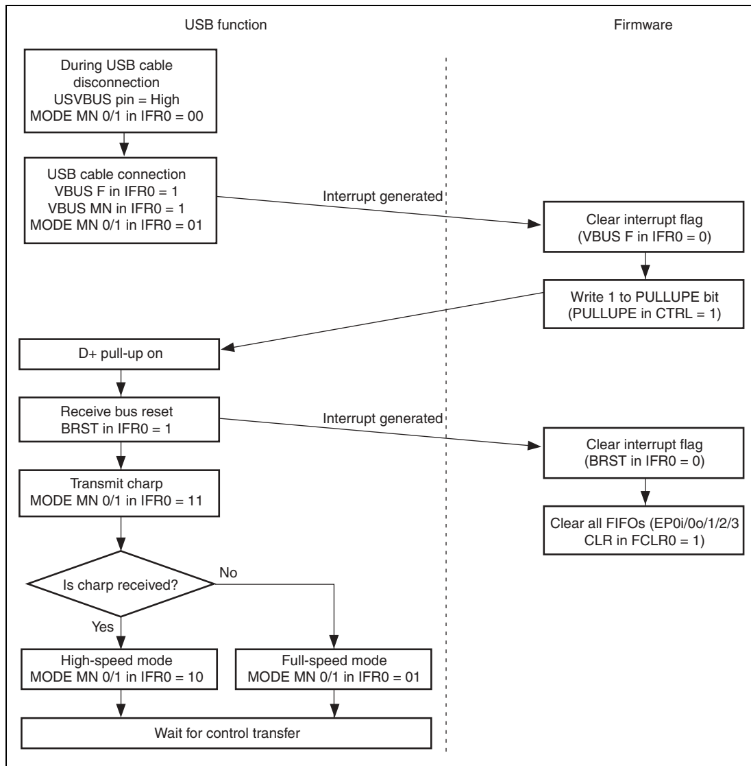
Figure 12.2 USB Cable Connection
