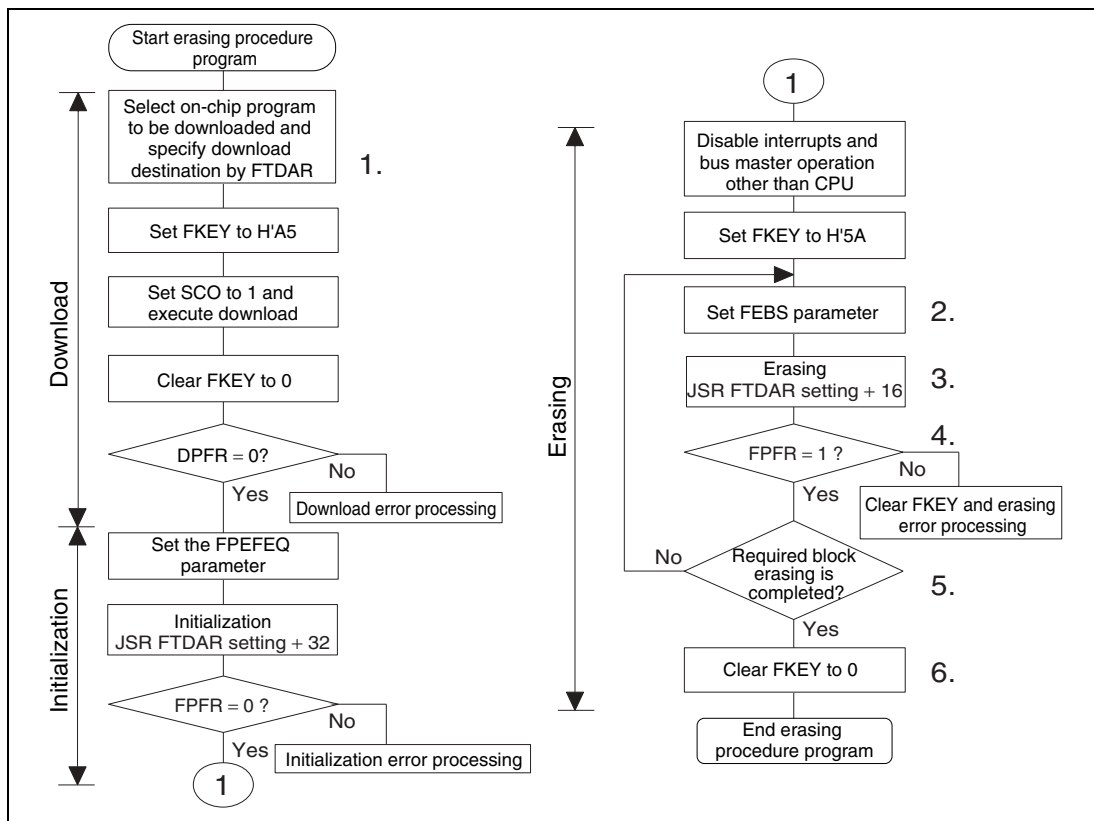
Figure 14.12 Erasing Procedure
