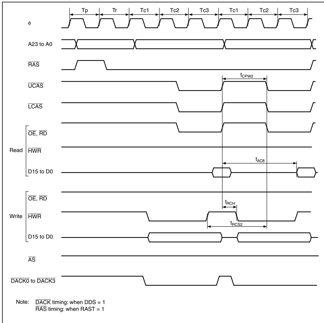
Figure 18.15 DRAM Access Timing: Three-State Burst Access
