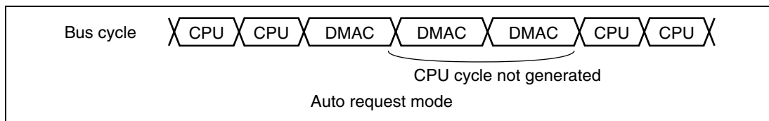
Figure 7.6 Examples of Timing in Burst Mode
