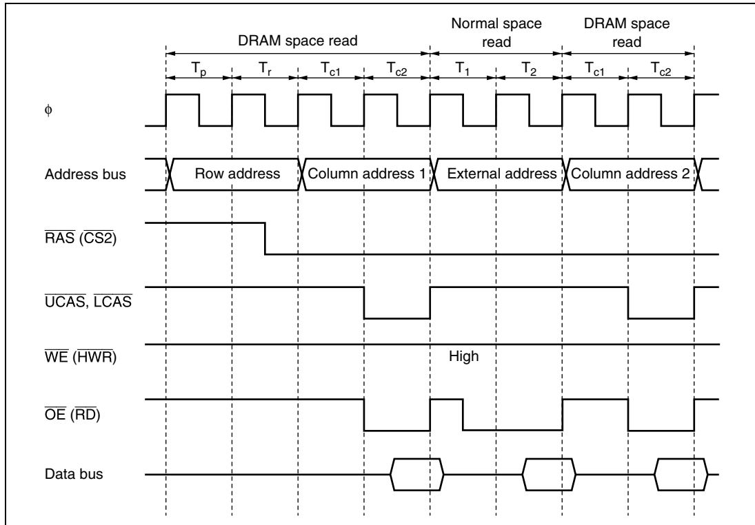
Figure 6.33 Example of Operation Timing in RAS Down Mode ( \text{RAST} = 0 , \text{CAST} = 0 )
