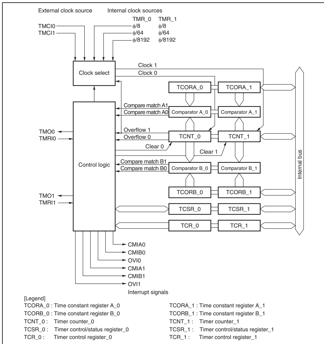
Figure 9.1 Block Diagram of 8-Bit Timer Module
