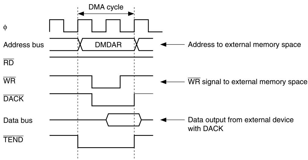
Figure 7.4 Example of Timing in Single Address Mode
