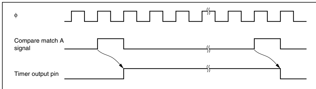
Figure 9.6 Timing of Timer Output
