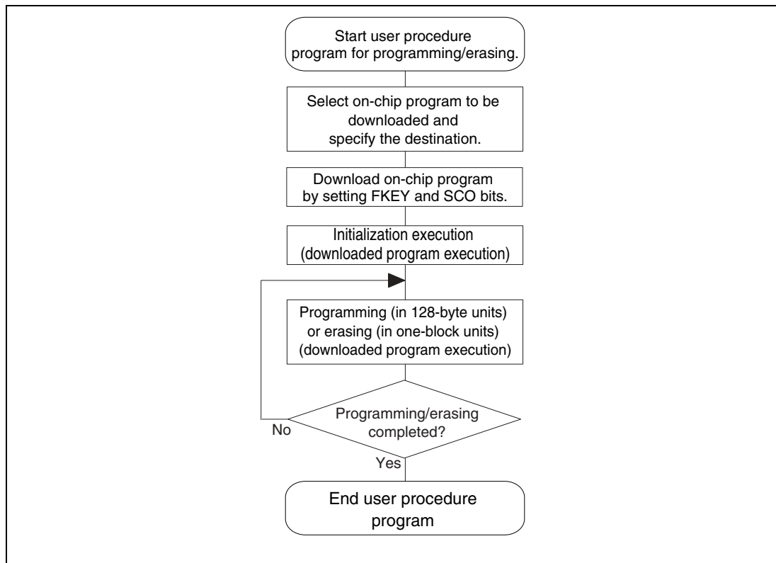
Figure 14.5 Overview of User Procedure Program
