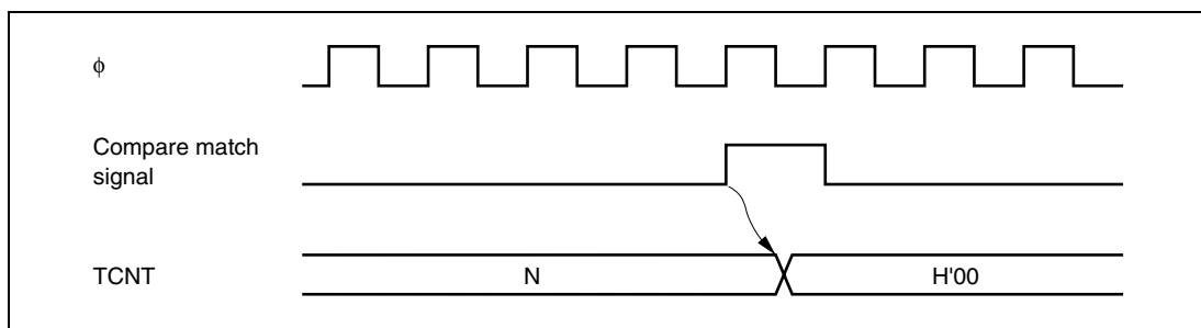
Figure 9.7 Timing of Compare Match Clear
