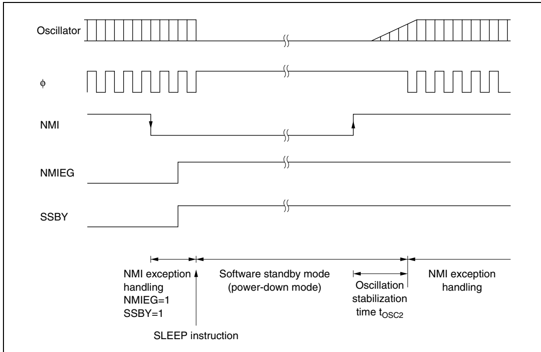
Figure 16.2 Software Standby Mode Application Example
