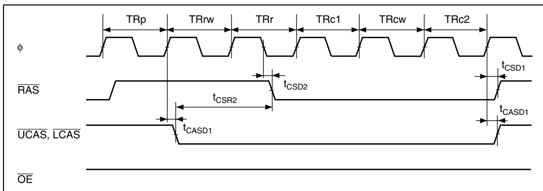
Figure 18.17 CAS-Before-RAS Refresh Timing (with Wait Cycle Insertion)
