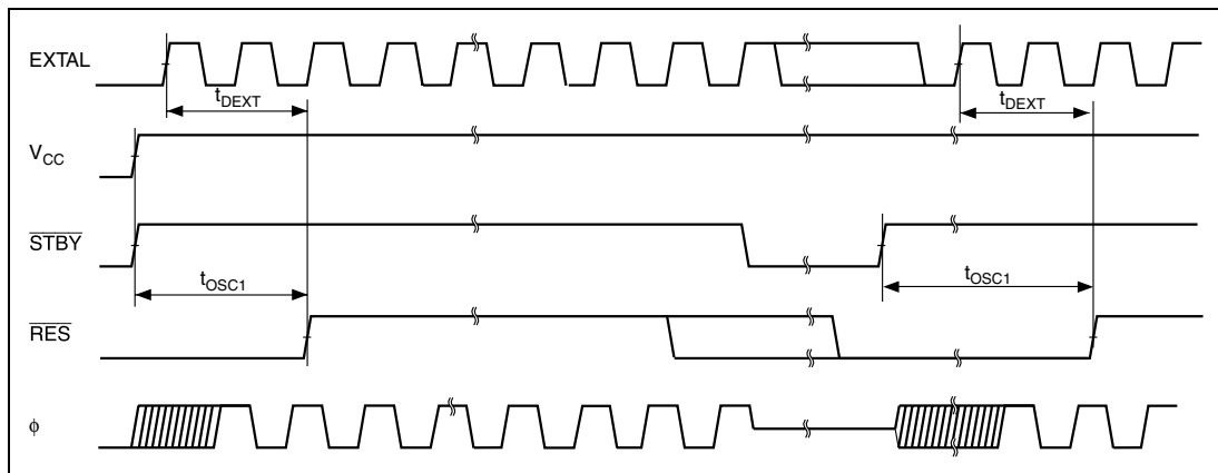
Figure 18.4 Oscillation Stabilization Timing (1)
