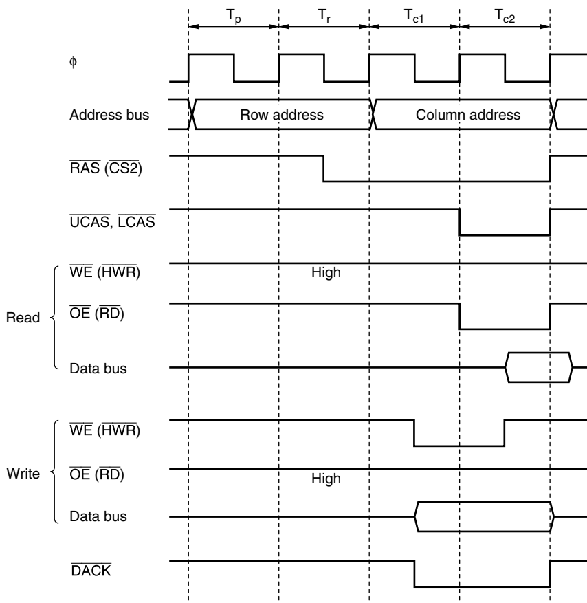
Figure 6.42 Example of \overline{\text{DACK}} Output Timing when \text{DDS} = 1 ( \text{RAST} = 0 , \text{CAST} = 0 )
