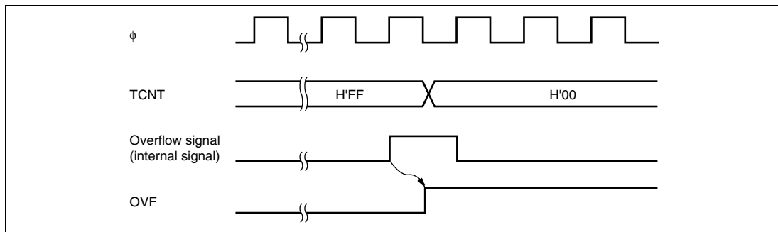
Figure 10.4 OVF Flag Set Timing
