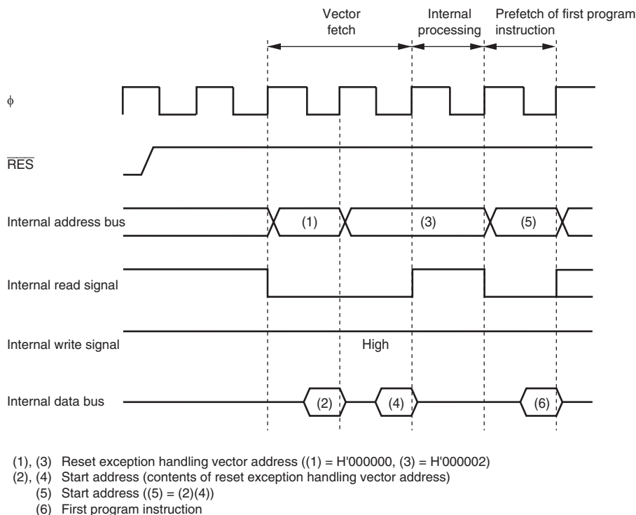
Figure 4.1 Reset Sequence
