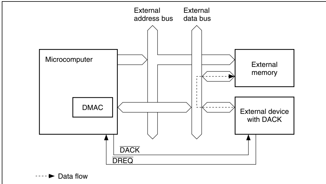
Figure 7.3 Data Flow in Single Address Mode
