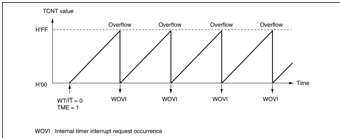
Figure 10.3 Interval Timer Mode Operation
