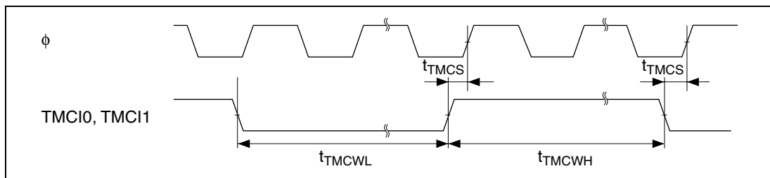
Figure 18.26 8-Bit Timer Clock Input Timing
