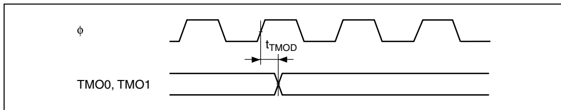
Figure 18.25 8-Bit Timer Output Timing
