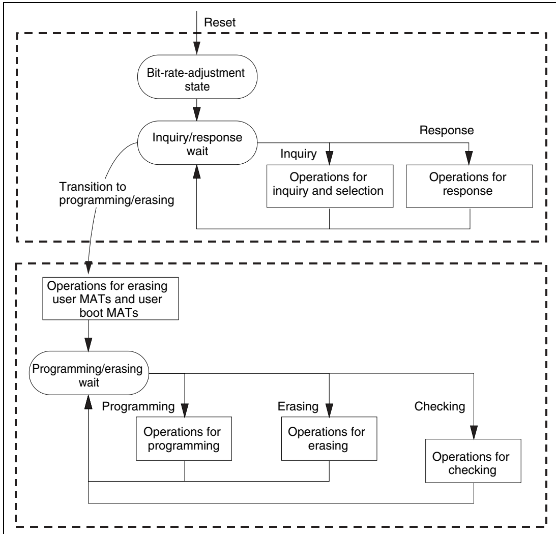
Figure 14.21 Boot Program States
