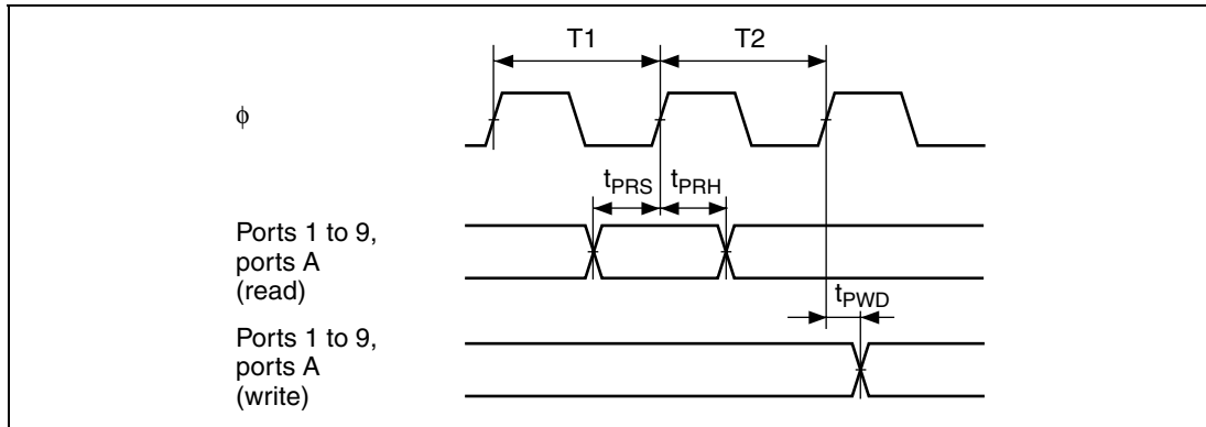
Figure 18.24 I/O Port Input/Output Timing
