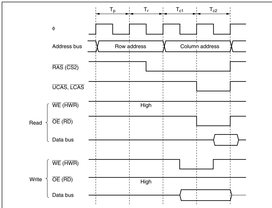
Figure 6.22 DRAM Basic Access Timing (RAST = 0, CAST = 0)
