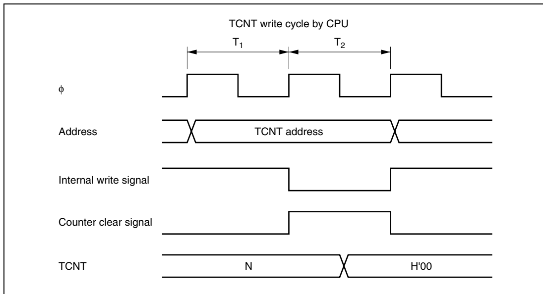
Figure 9.10 Contention between TCNT Write and Clear
