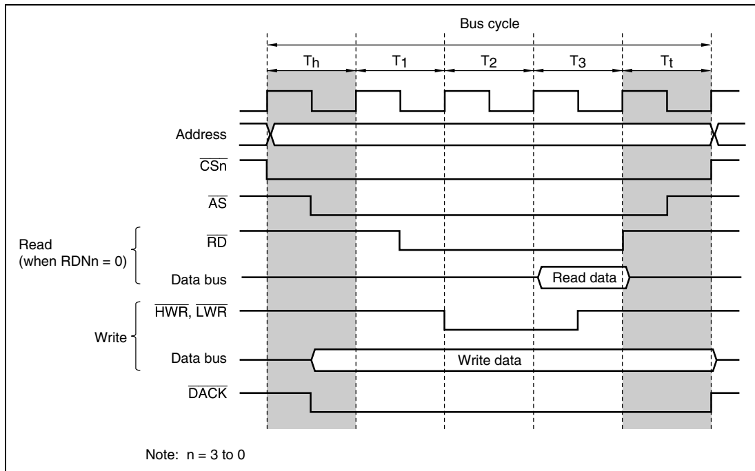
Figure 6.2 \overline{CS} and Address Assertion Period Extension (Example of 3-State Access Space and RDNn = 0 )
