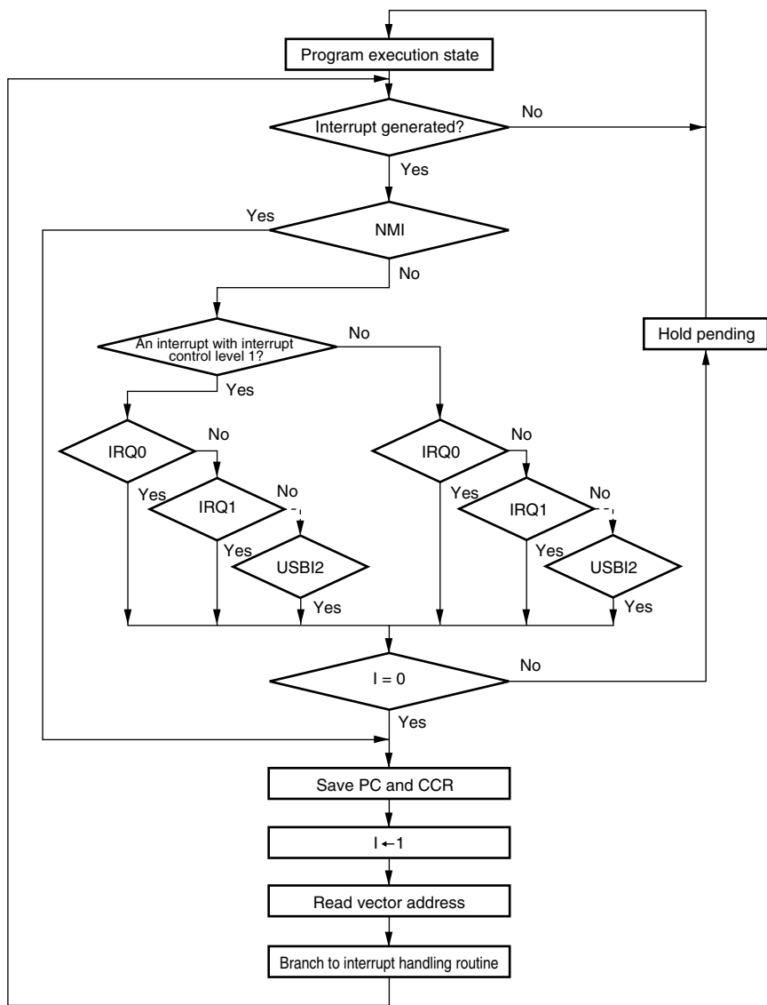
Figure 5.4 Flowchart of Procedure up to Interrupt Acceptance in Interrupt Control Mode 0
