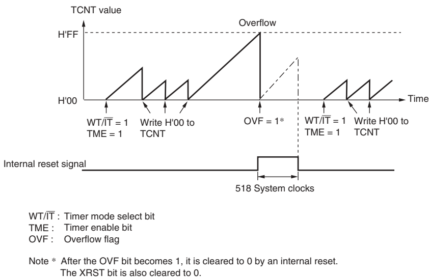
Figure 10.2 Watchdog Timer Mode ( \overline{RST}/\overline{NMI} = 1 ) Operation
