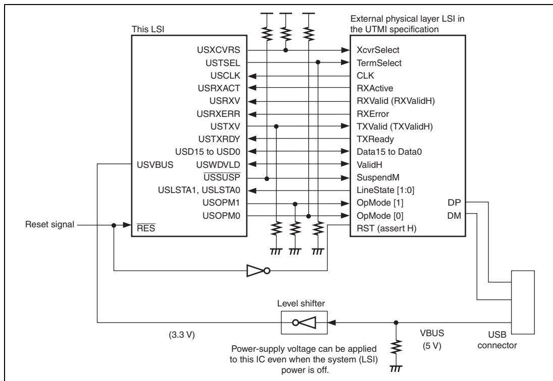
Figure 12.18 Connection Example of External Circuit
