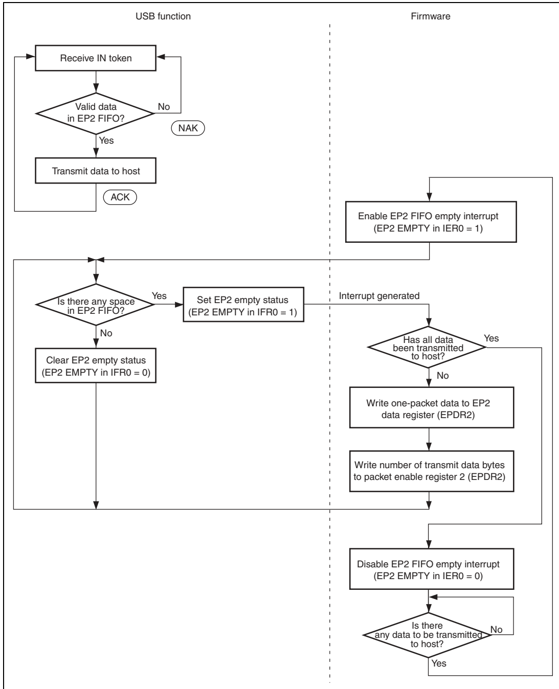
Figure 12.11 EP2 Bulk-In Transfer Operation
