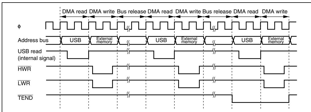
Figure 7.17 Example of Normal Transfer Mode (Cycle Steal Mode) Transfer (Transfer Source: USB)
