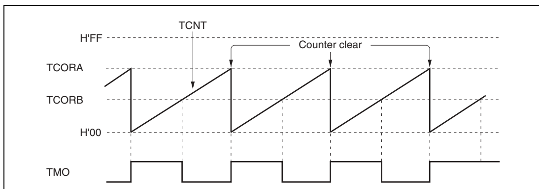
Figure 9.2 Example of Pulse Output
