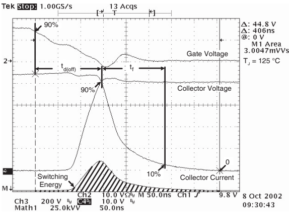
Figure 23, Turn-off Switching Waveforms and Definitions
