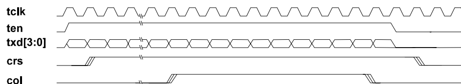
Figure 23. Transmission with Collision Timing
