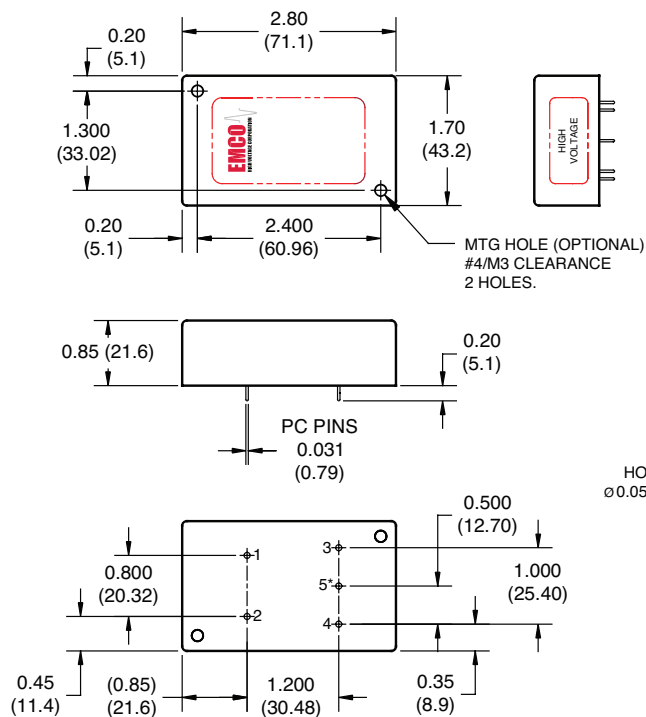
TOP VIEW
