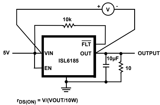
FIGURE 29A. r_{DS(ON)}
