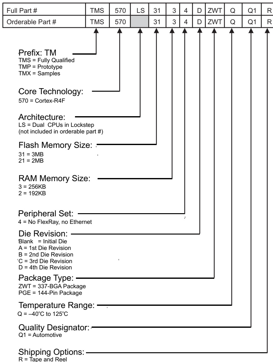
Figure 8-1. TMS570LS31x4/21x4 Device Numbering Conventions
