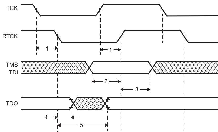
Figure 6-22. JTAG Timing
