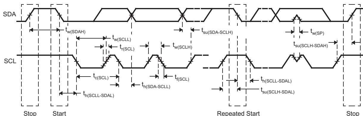
Figure 7-8. I2C Timings
