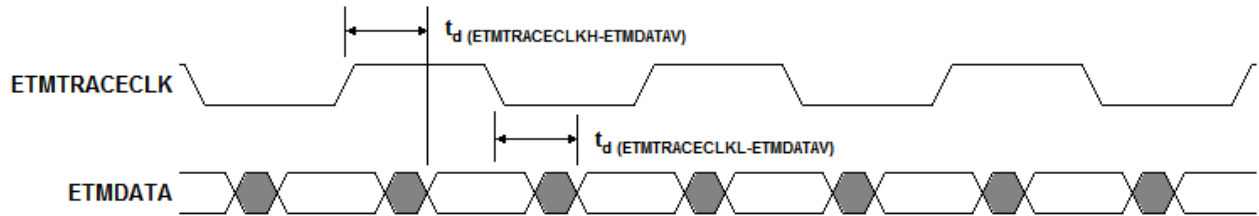
Figure 6-25. ETMDATA Timing
