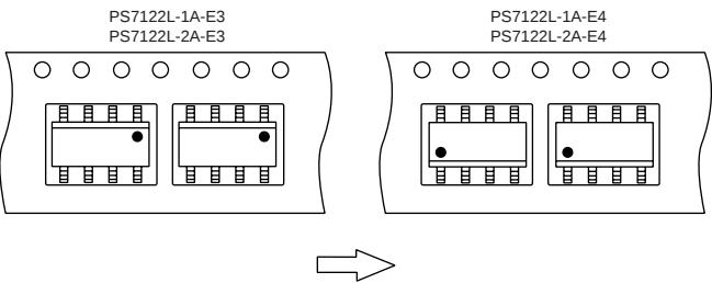
TAPING DIRECTION
