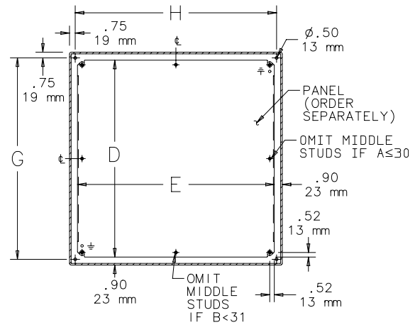
SECTION Y-Y (WITH PANEL INSTALLED)
