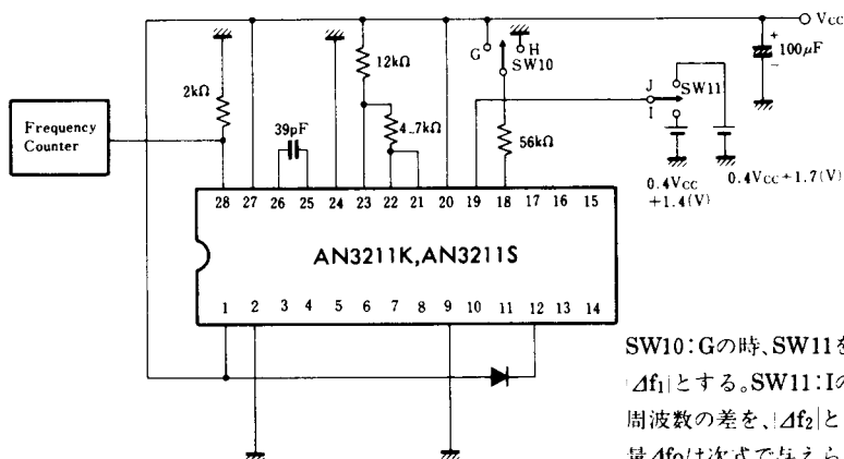
Test Circuit 9 ( \Delta f_0 )
