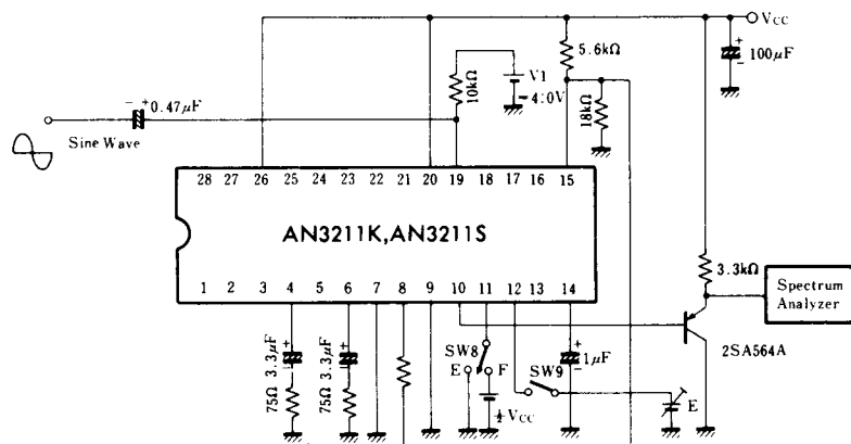
Test Circuit 9 ( \Delta f_0 )
