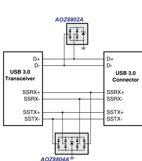
Figure 1. USB 3.0 Ports
