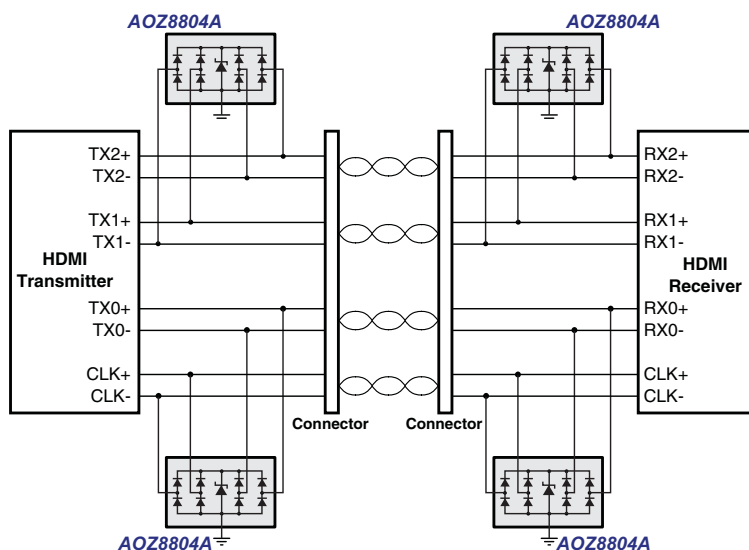
Figure 2. HDMI Ports
