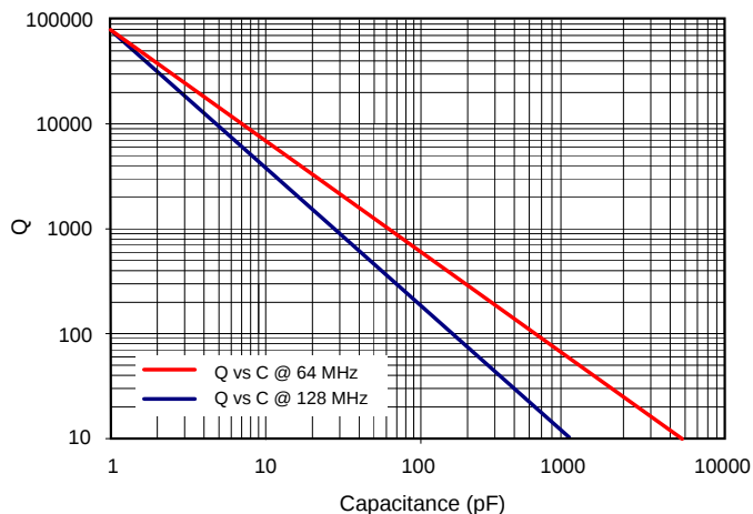
S48E Q vs. Capacitance, Typical (Preliminary)
