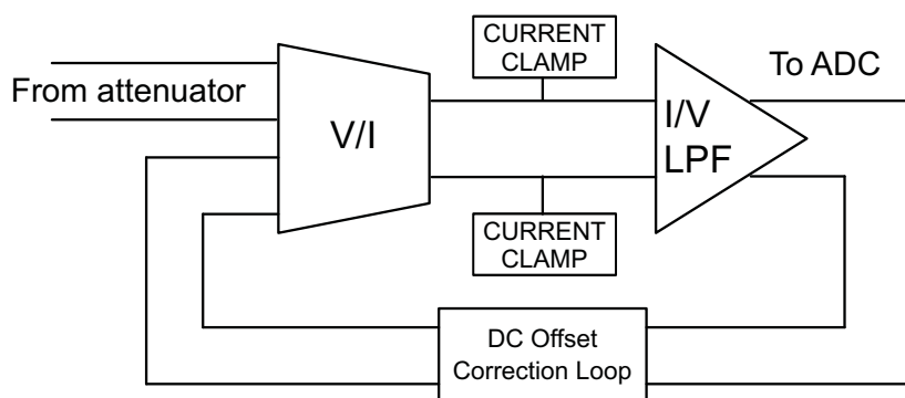
Figure 68. Simplified Block Diagram of PGA
