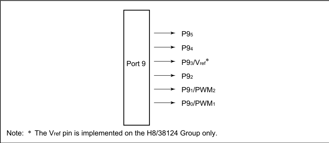
Figure 8.8 Port 5 Pin Configuration
