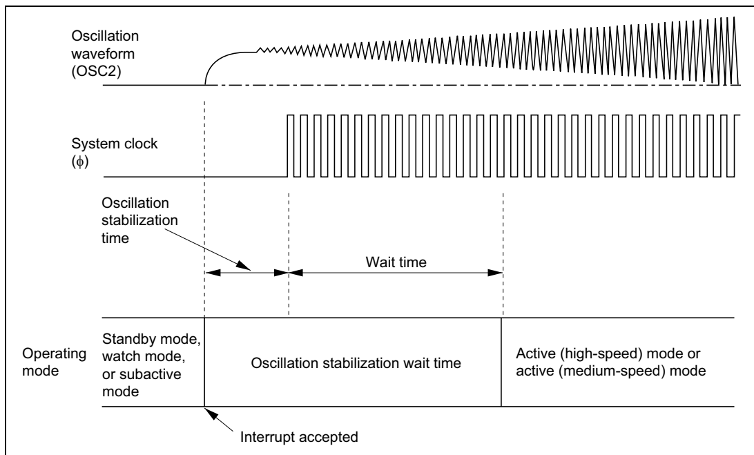
Figure 4.14 Oscillation Stabilization Wait Time
