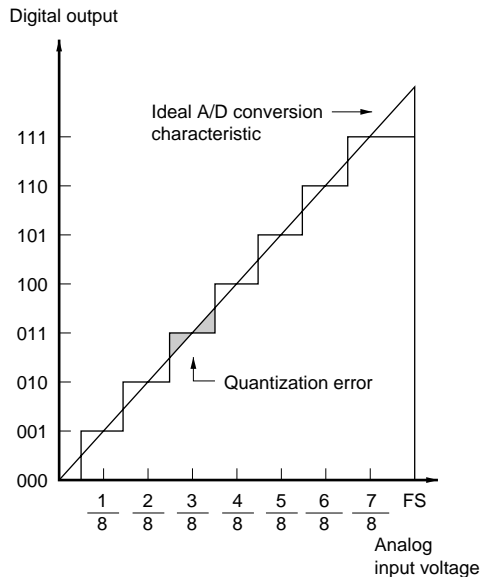
Figure 12.6 A/D Conversion Accuracy Definitions (1)
