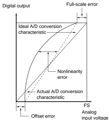
Figure 12.7 A/D Conversion Accuracy Definitions (2)
