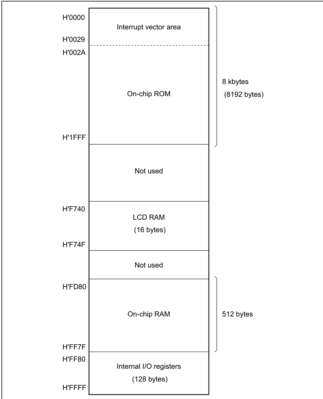
Figure 2.16(5) H8/38020, H8/38020S, and H8/38120 Memory Map
