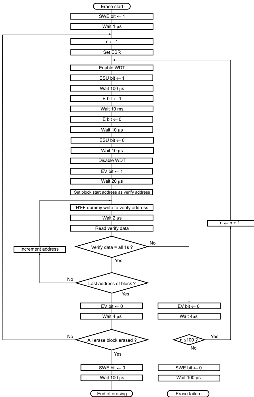
Figure 6.11 Erase/Eraser-Verify Flowchart
