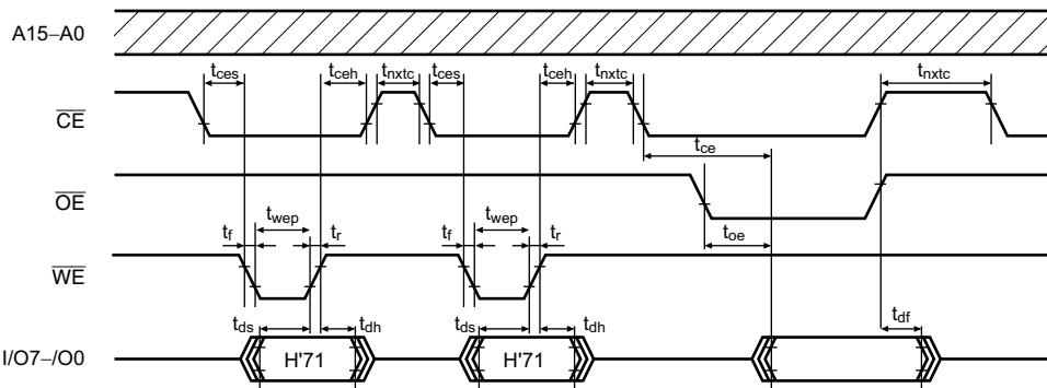
Figure 6.19 Status Read Mode Timing Waveforms
