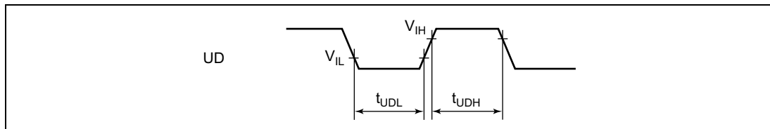
Figure 16.6 UD Pin Minimum Transition Width Timing
