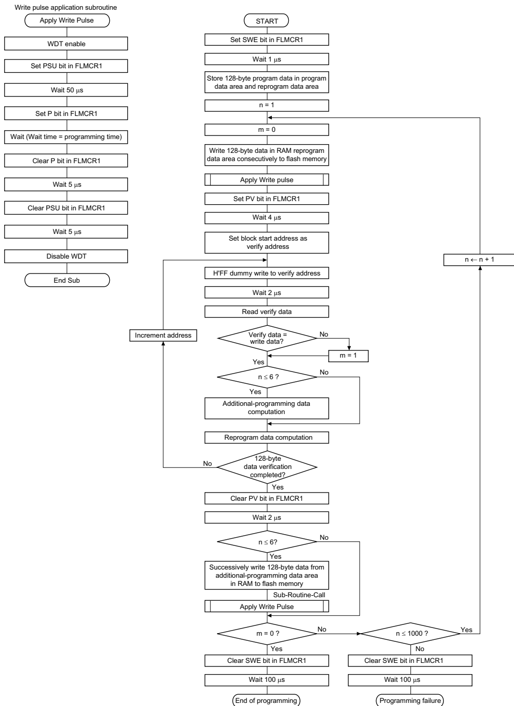
Figure 6.10 Program/Program-Verify Flowchart
