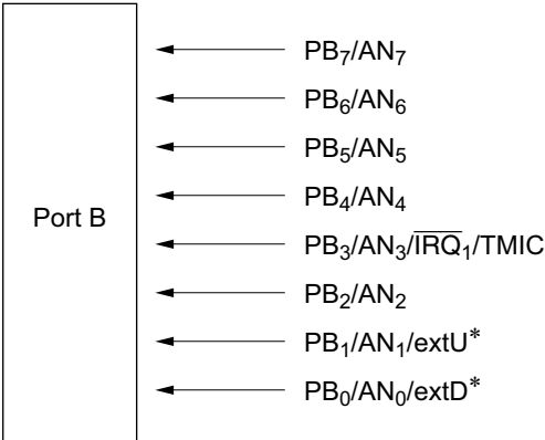
Figure 8.10 Port B Pin Configuration
