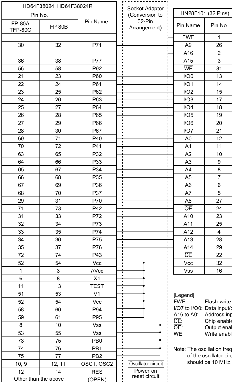
Figure 6.12(1) Socket Adapter Pin Correspondence Diagram (HD64F38024, HD64F38024R)
