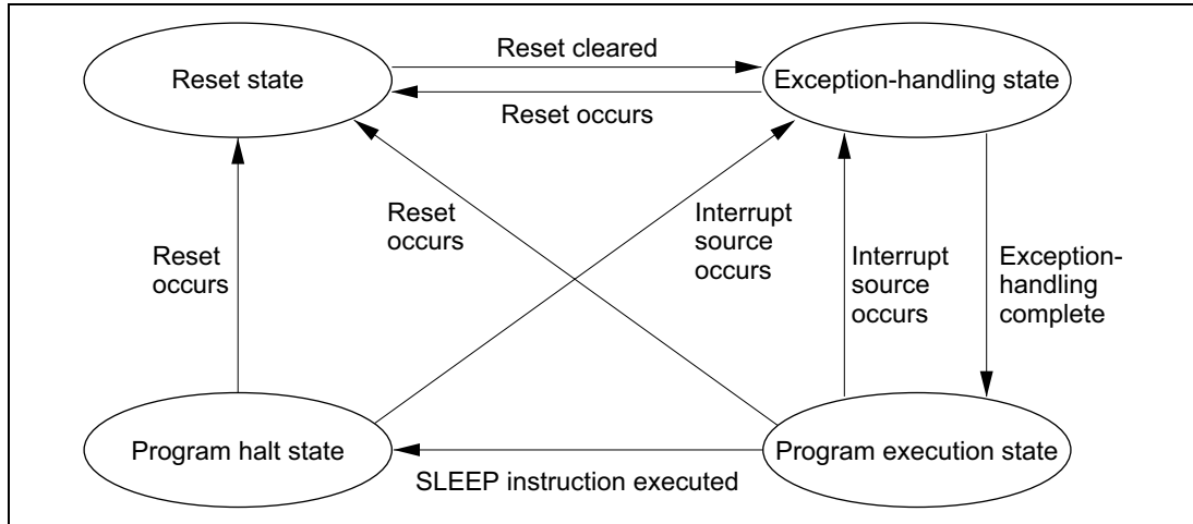
Figure 2.15 State Transitions
