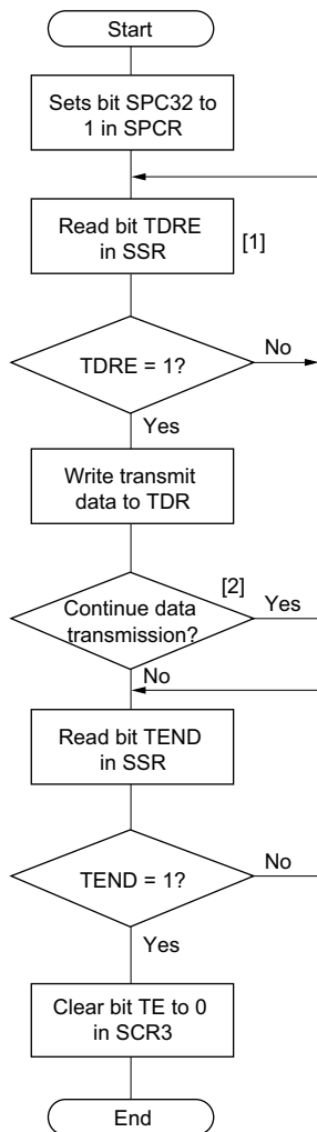
Figure 10.11 Example of Data Transmission Flowchart (Synchronous Mode)
