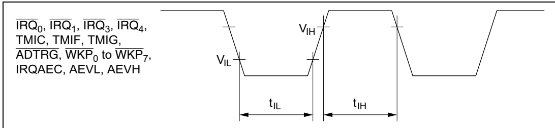
Figure 16.3 Input Timing
