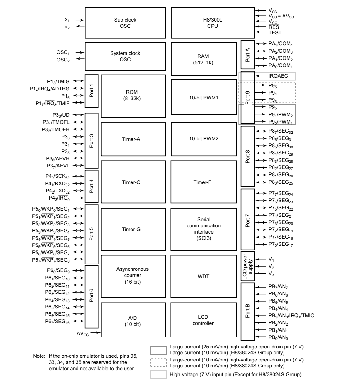
Figure 1.1(1) Block Diagram (H8/38024 Group, H8/38024S Group)
