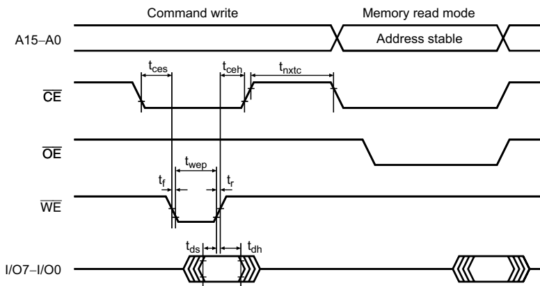
Figure 6.13 Timing Waveforms for Memory Read after Memory Write
