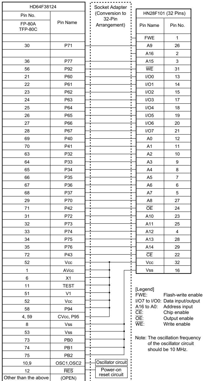
Figure 6.12(2) Socket Adapter Pin Correspondence Diagram (HD64F38124)
