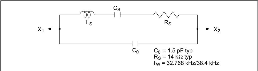
Figure 4.9 Equivalent Circuit of 32.768 kHz/38.4 kHz Crystal Oscillator
