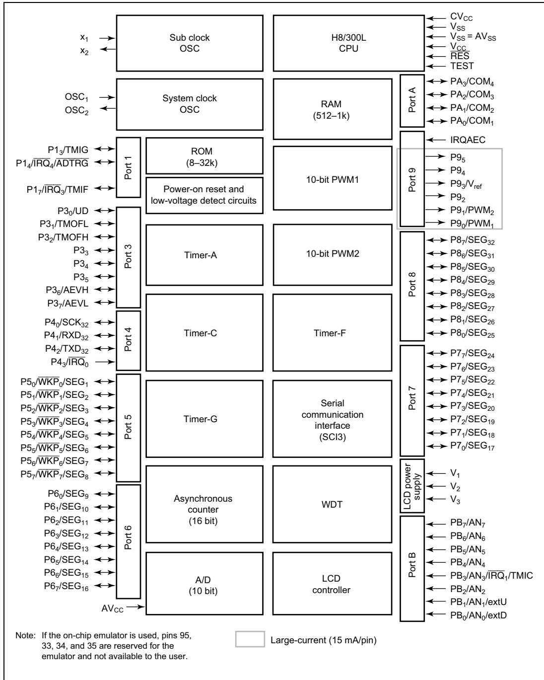
Figure 1.1(2) Block Diagram (H8/38124 Group)
