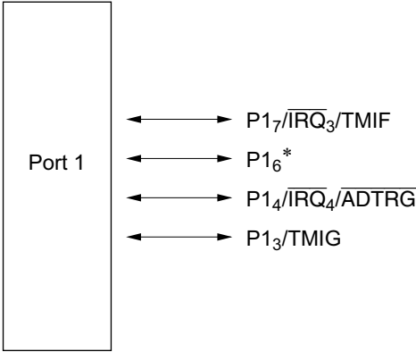
Figure 8.1 Port 1 Pin Configuration
