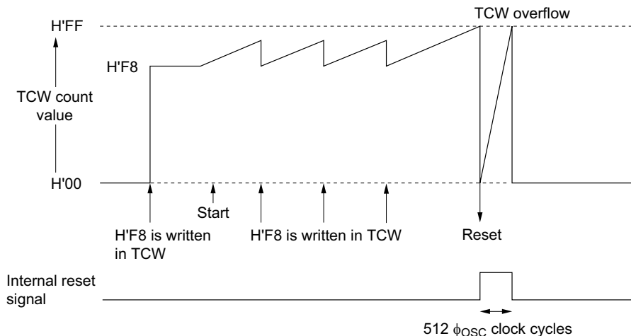
Figure 9.18 Typical Watchdog Timer Operations (Example)
