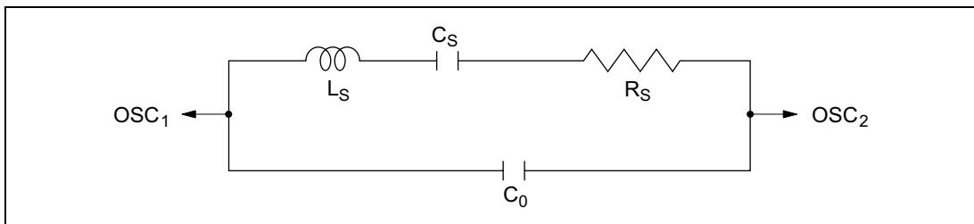
Figure 4.4 Equivalent Circuit of Crystal Oscillator
