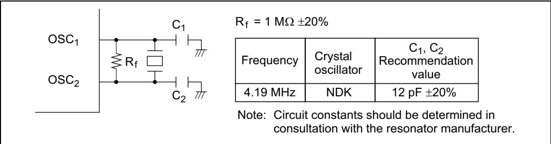
Figure 4.3(1) Typical Connection to Crystal Oscillator (H8/38024, H8/38024F-ZTAT Group)
