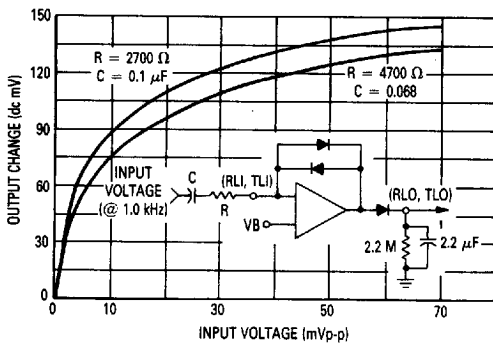
FIGURE 8 — LOG AMP TRANSFER CHARACTERISTICS
