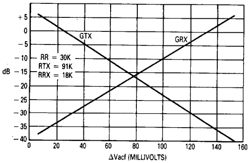
FIGURE 6 — ATTENUATOR GAIN versus \Delta V_{ac}
