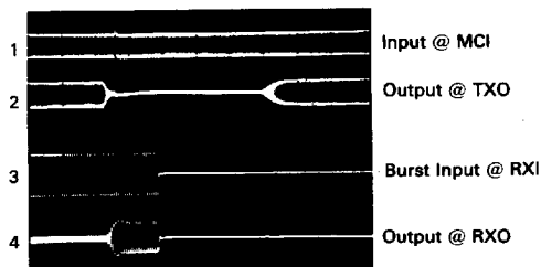
FIGURE 17 — IDLE-RECEIVE SWITCHING
