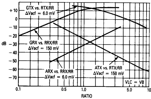
FIGURE 4 — GAIN AND ATTENUATION versus RESISTOR RATIOS
