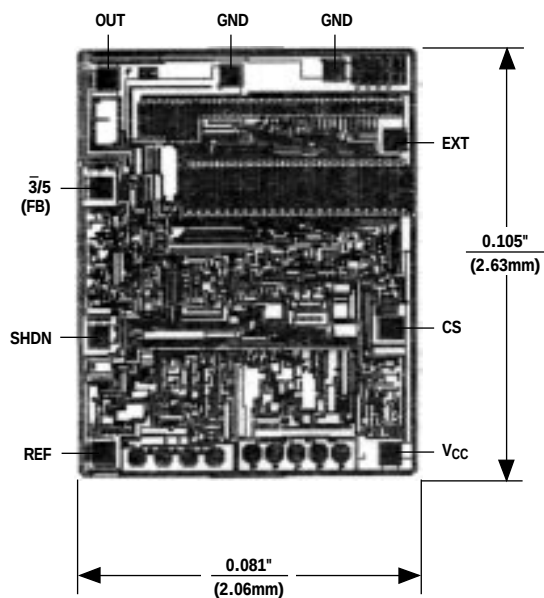
Chip Topography
