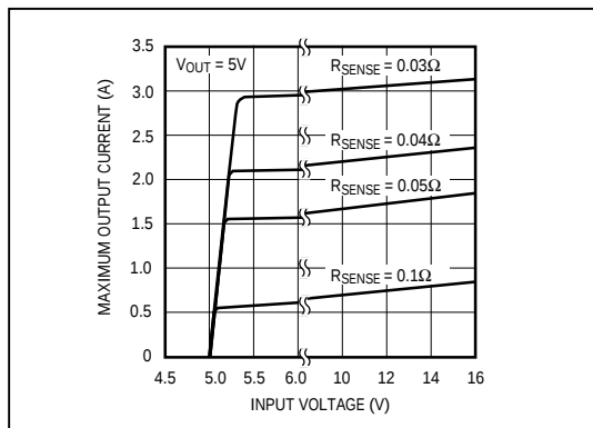
Figure 6a. MAX1626 5V-Operation Current-Sense Resistor Graph
