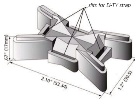
El-Ty Spacer
