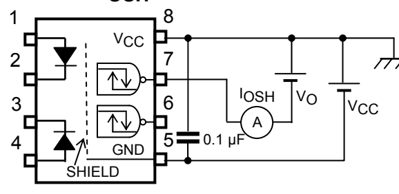
TEST CIRCUIT 6: I_{OSH} Test Circuit
