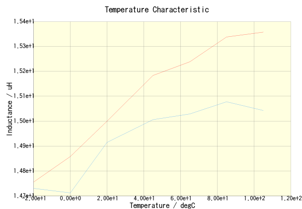
VLF403215MT-150M-CA(DC = 0A) VLF403215MT-150M-CA(DC = 0.39A)
