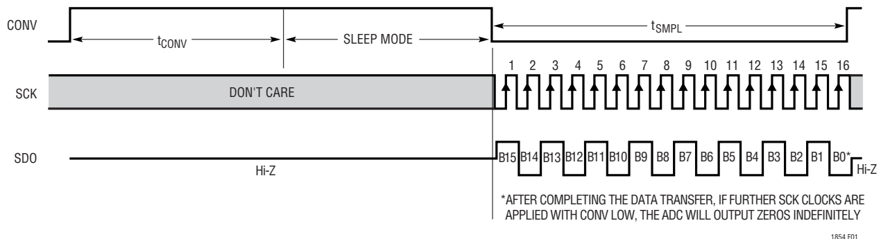
Figure 1. LTC1864L Operating Sequence
