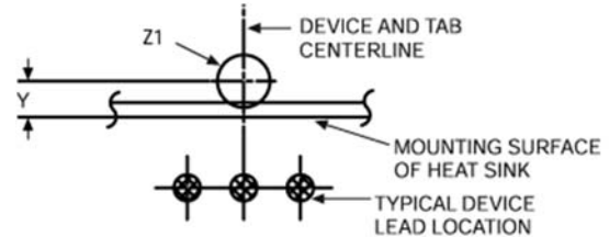
Mounting Details:
