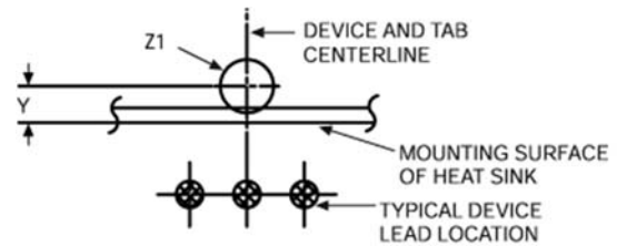
Mounting Details:
