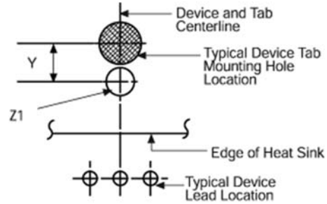
Mounting Details:
