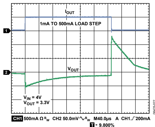
Figure 24. Load Transient Response, C_{OUT} = 1\text{ }\mu\text{F}
