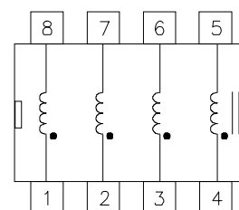
F-135X Schematic
