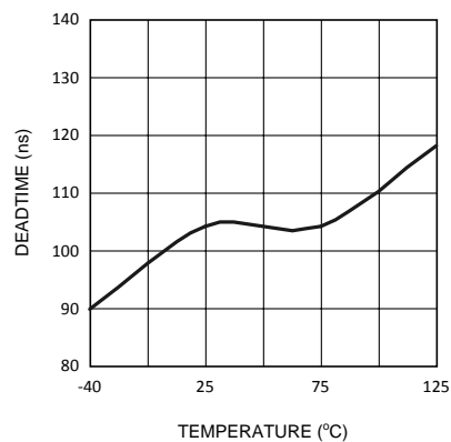
Figure 8. Dead Time vs Temperature RSET = 29.5 kΩ
