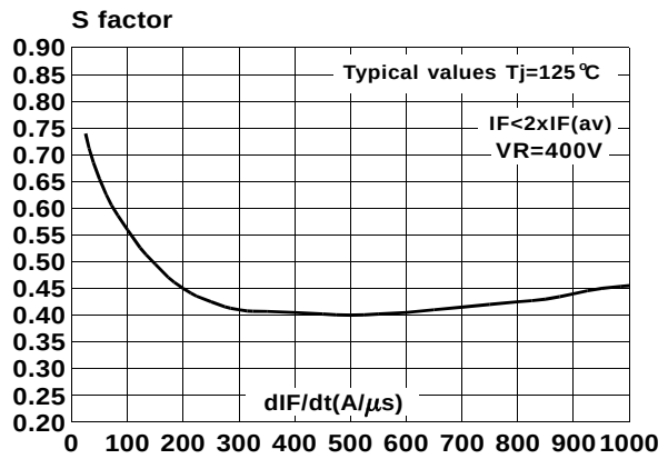
Fig. 6: Softness factor ( t_b/t_a ) versus dl_F/dt .
