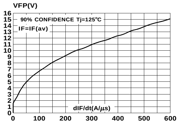
Fig. 8: Transient peak forward voltage versus dl_F/dt .
