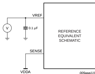
Fig 14. External reference, 1 V (p-p) to 2 V (p-p) full-scale
