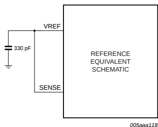
Fig 13. Internal reference via SPI, 1 V (p-p) to 2 V (p-p) full-scale
