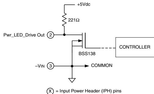
Typical Power Good External LED Lamp Wiring
