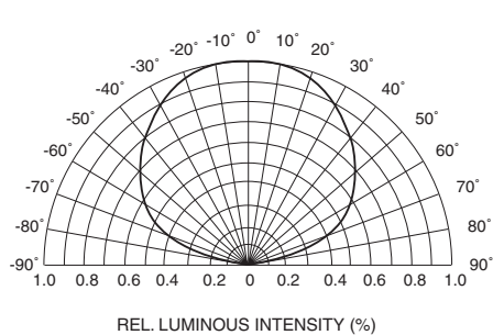
Fig. 4 Radiation Diagram
