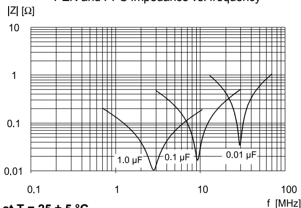
PEN and PPS Impedance vs. frequency
