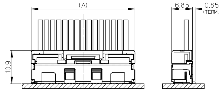
嵌合図 MATED CONNECTORES (SCALE : 2-1)
