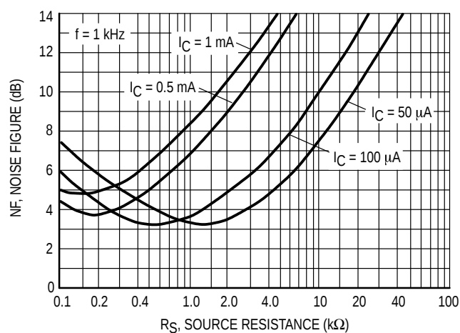
Figure 4. Source Resistance
