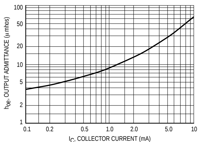
Figure 6. Output Admittance
