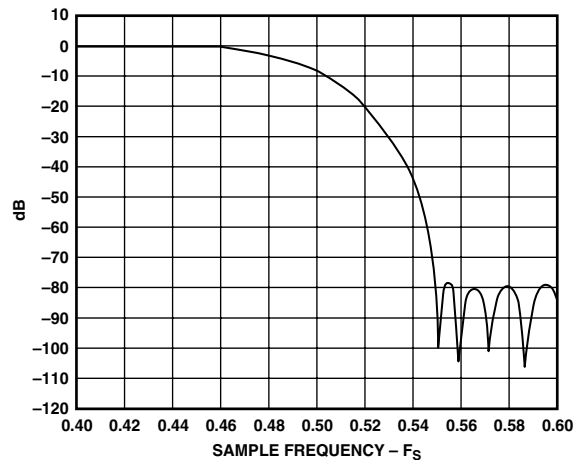
Figure 27. Digital-to-Analog Frequency Response—Transition Band (Full-Scale Inputs, 0 dB Attenuation)
