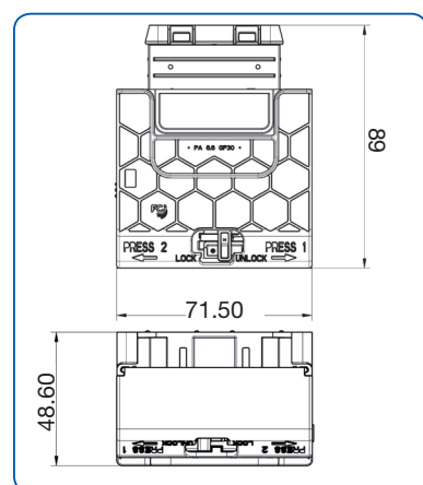
Female plug
