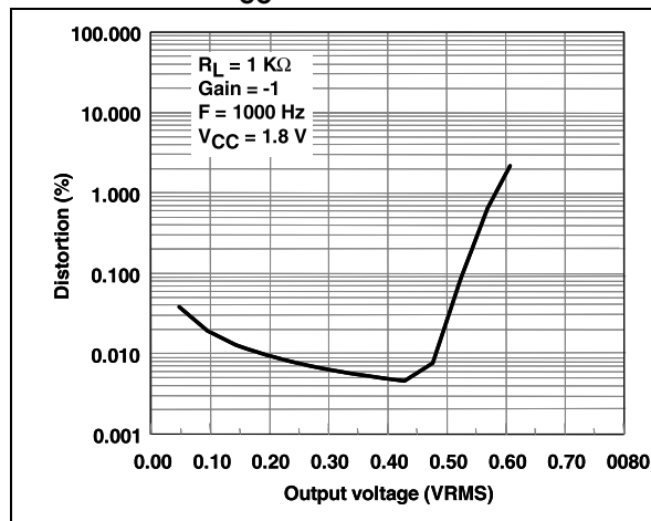
Figure 37. Distortion vs. output voltage at V_{CC} = 1.8\text{ V}
