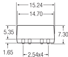
10 PIN SMD Package
