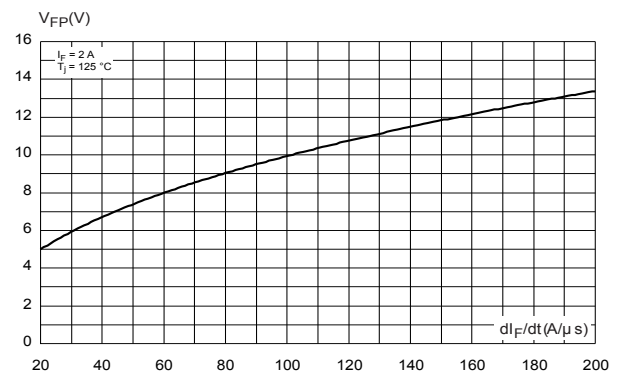
Figure 10. Transient peak forward voltage versus dl_F/dt (typical values)
