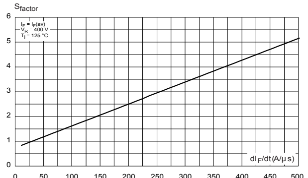
Figure 8. Reverse recovery softness factor versus dl_F/dt (typical values)
