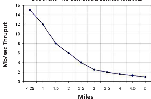
Q-Bridge+ Typical Thruput vs Distance Line of Site = No Obstructions Between Antennas
