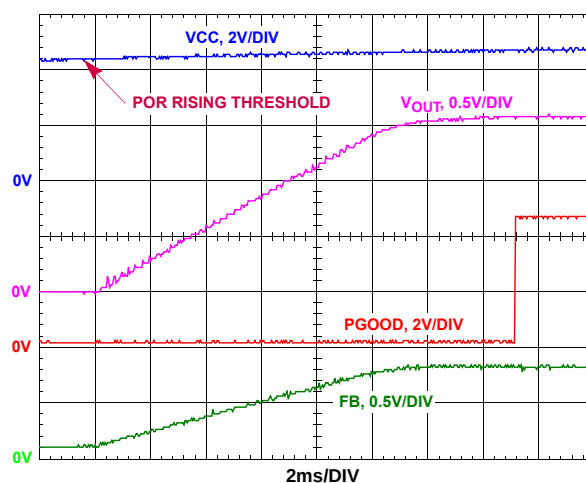
FIGURE 3. SOFT-START WAVEFORMS
