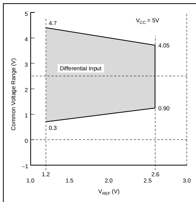
Figure 22. Differential Input: Common-Mode Voltage Range vs V_{REF}
