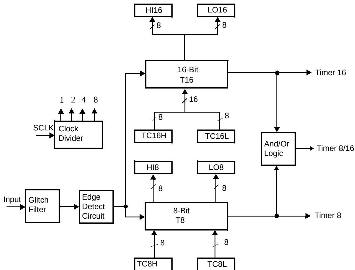
Figure 2. Counter/Timers Diagram
