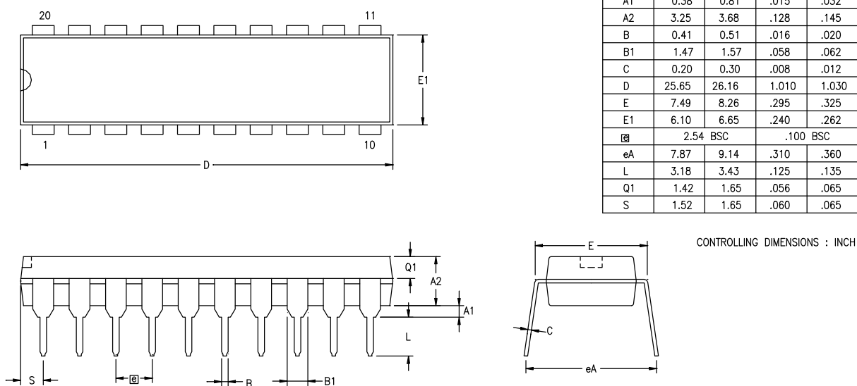
Figure 55. 20-Pin DIP Package Diagram
