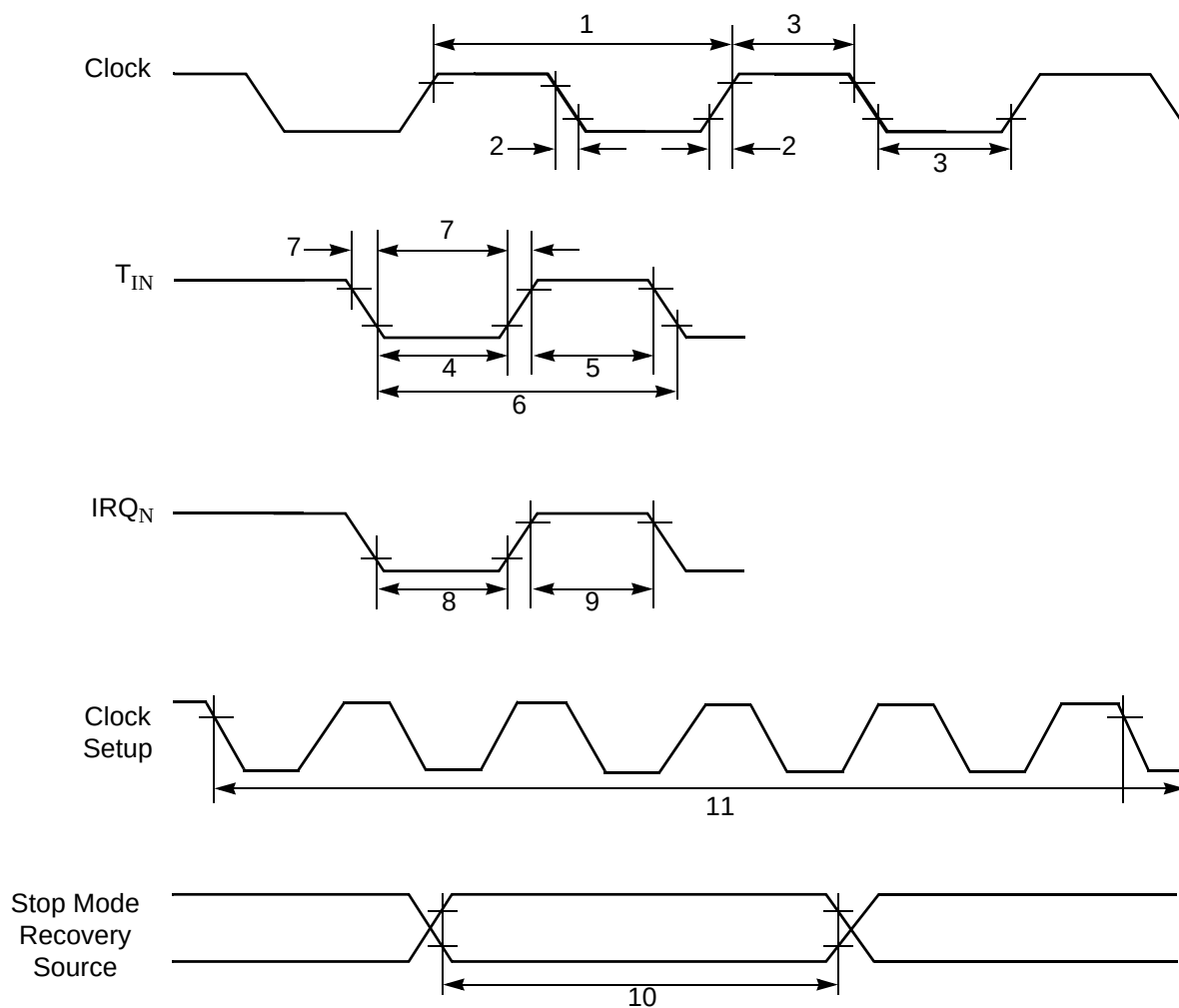
Figure 54. AC Timing Diagram
