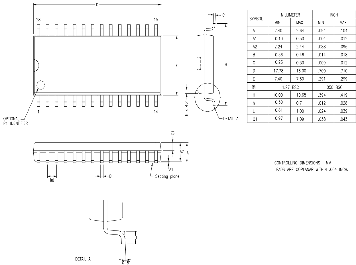
Figure 58. 28-Pin SOIC Package Diagram
