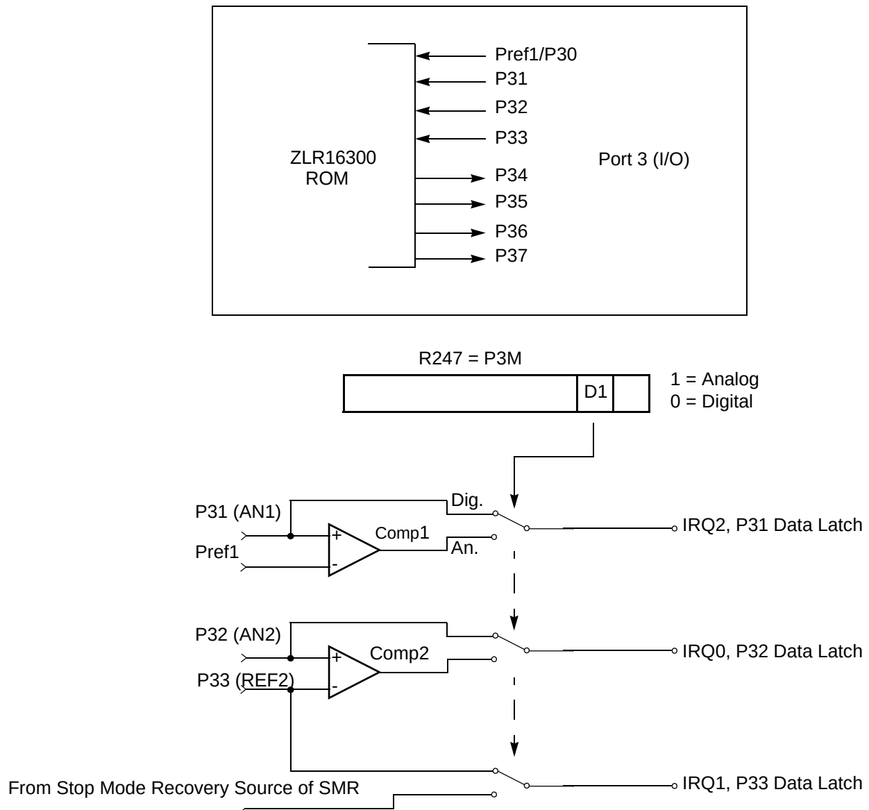
Figure 7. Port 3 Configuration
