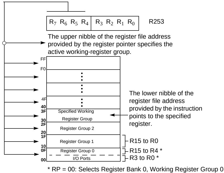
Figure 12. Register Pointer—Detail
