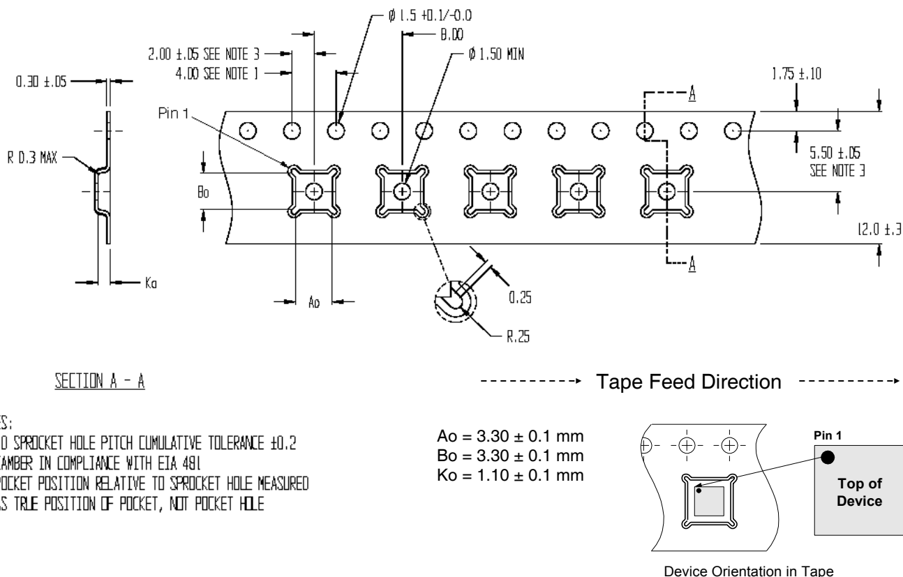
Figure 23. Tape and Reel Specifications
