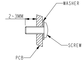
DETAIL 2 RECOMMENDED SCREW LENGTH
