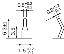
(Terminal dimensions)
