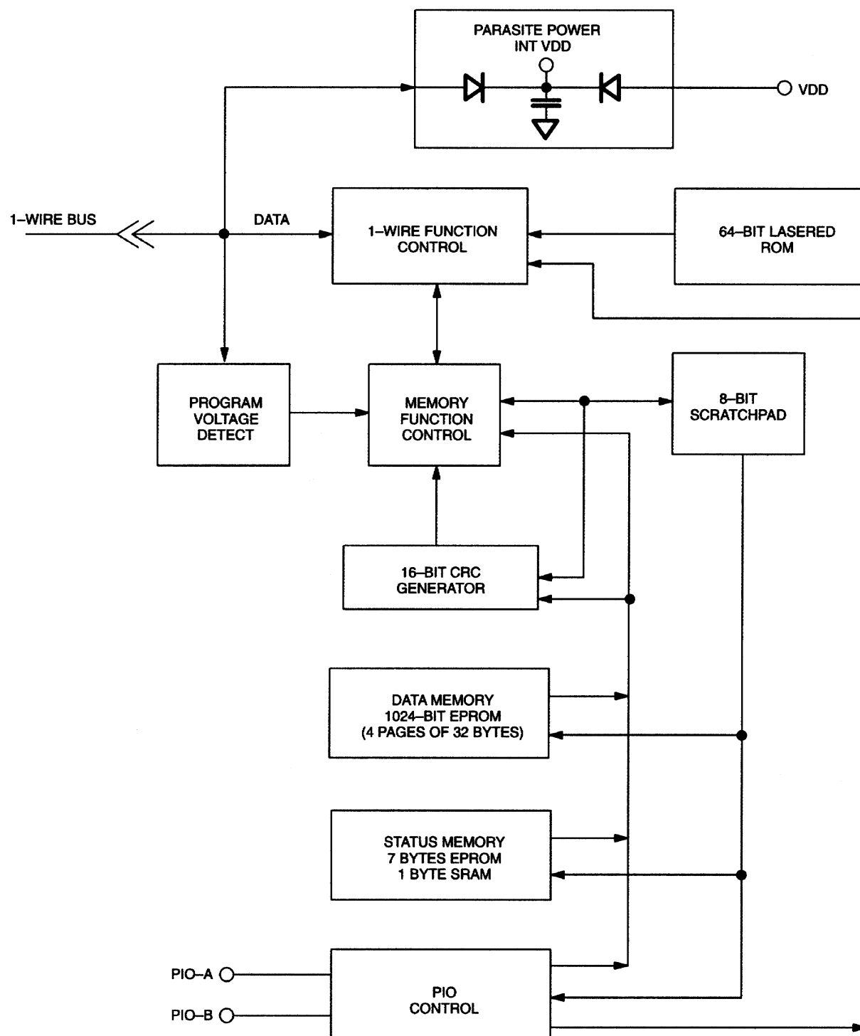
DS2407 BLOCK DIAGRAM Figure 1
