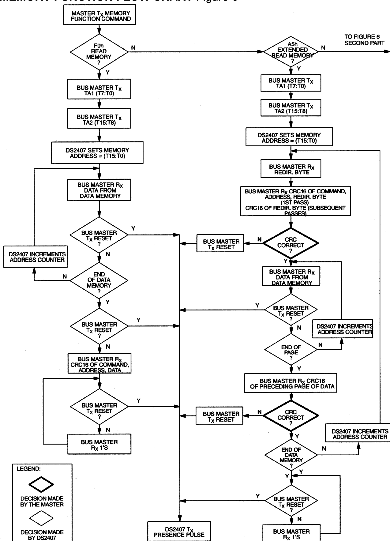
MEMORY FUNCTION FLOW CHART Figure 6
