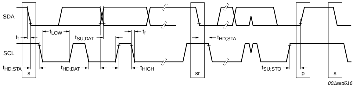
Fig 11. Timing diagram
