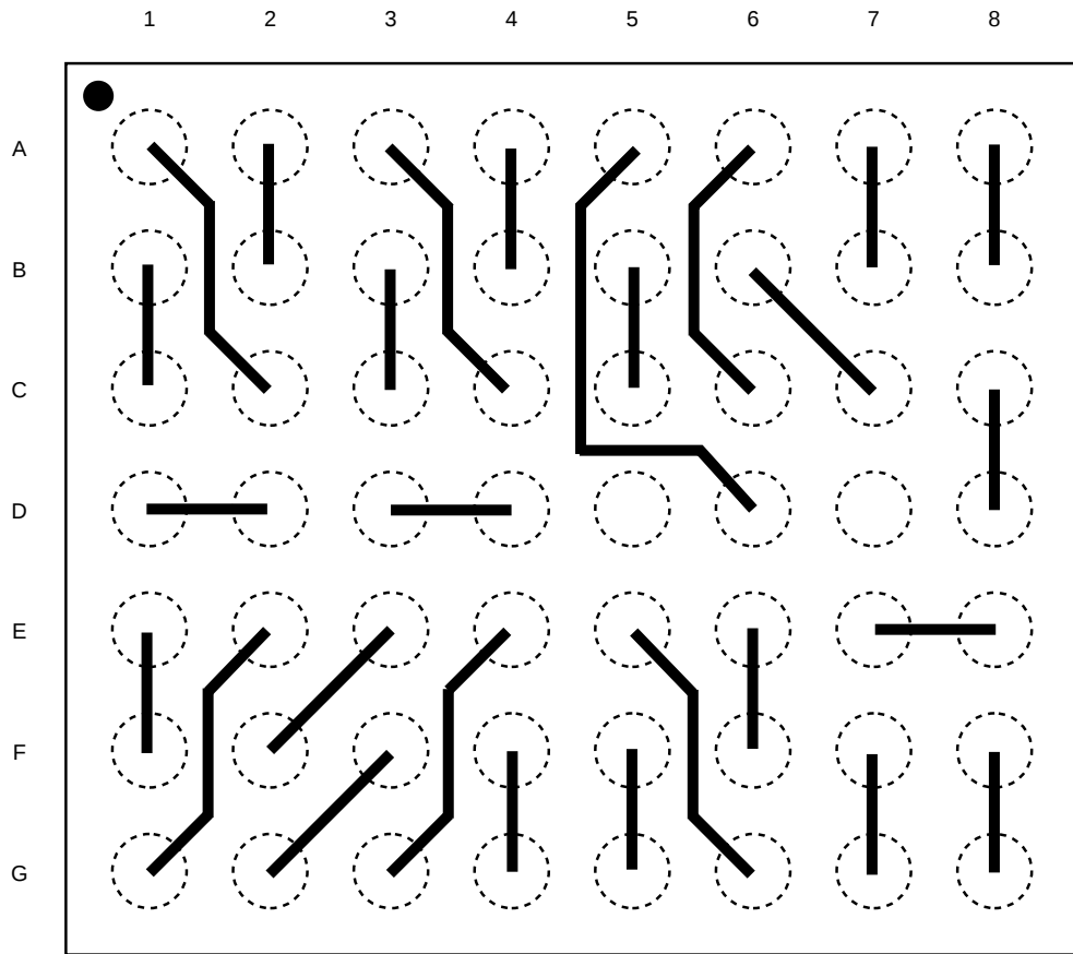
Figure 18. TFBGA56 Daisy Chain - Package Connections (Top view through package)
