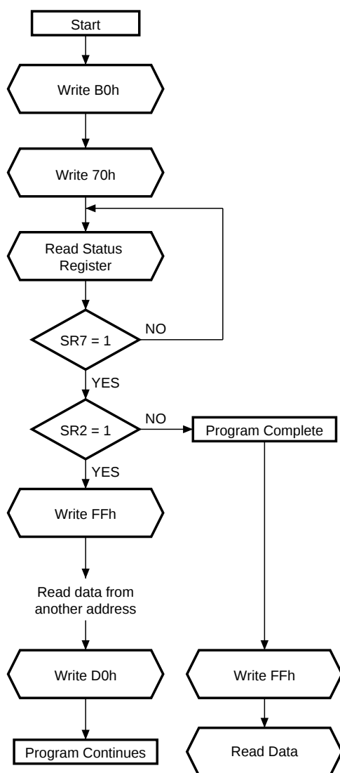
Figure 23. Program Suspend &amp; Resume Flowchart and Pseudo Code
